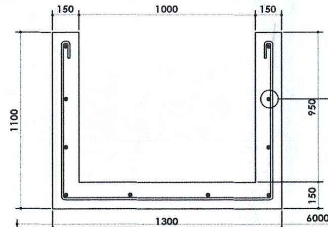
DETAIL OF FLUME
