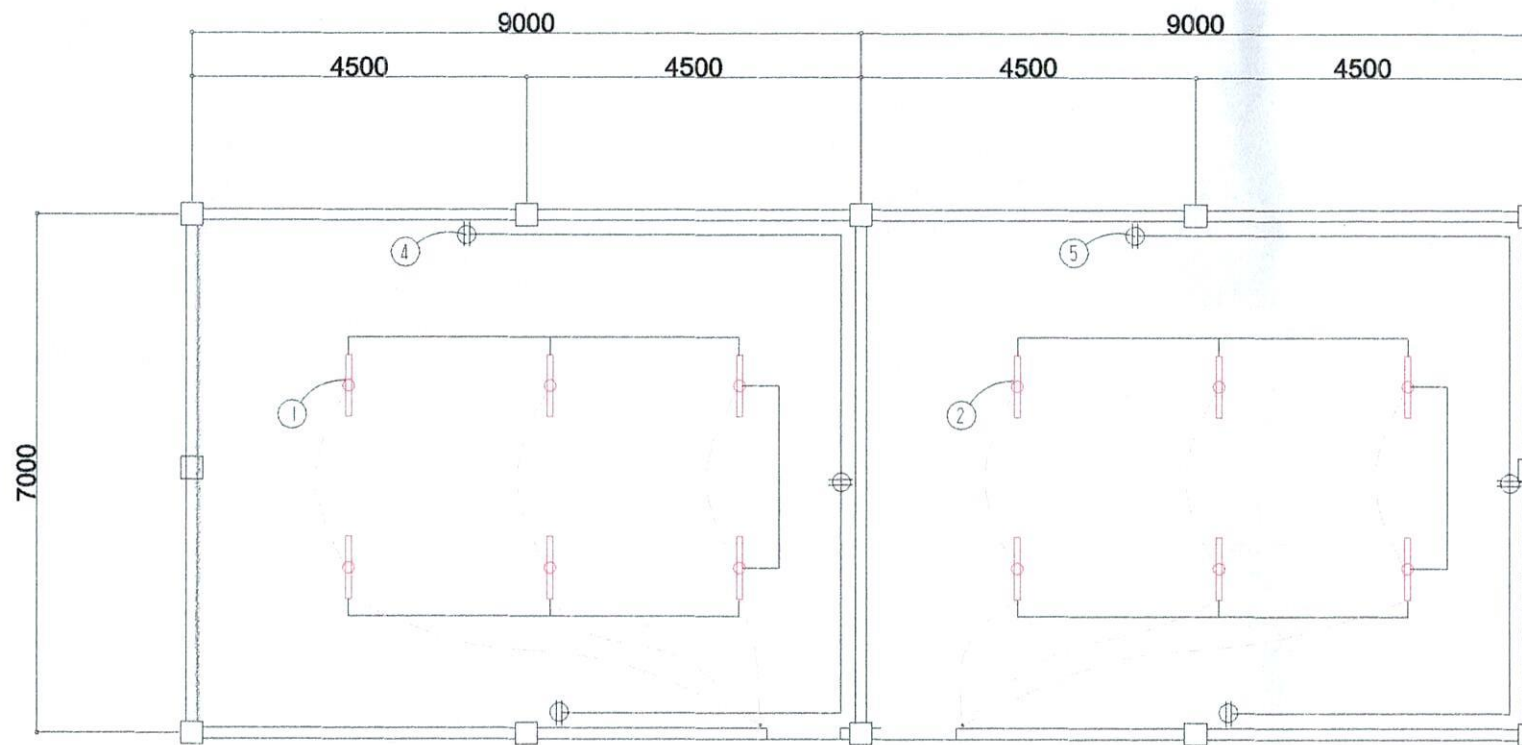
ELECTRICAL PLAN SCALE: 1/25HTS
