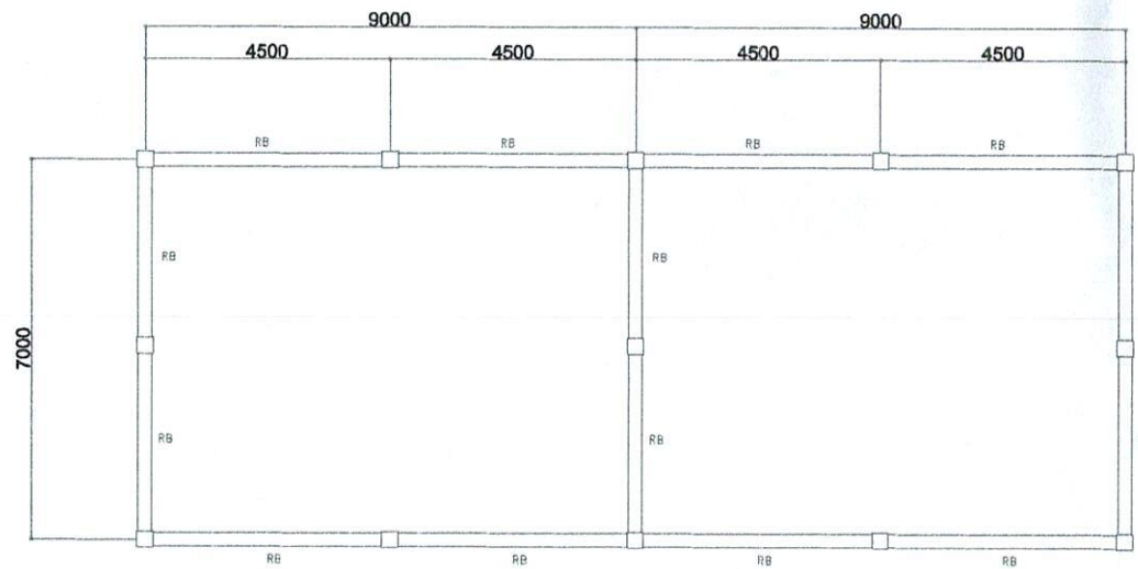
ROOF BEAM LAYOUT SCALE: 1/8"=1'-0"
