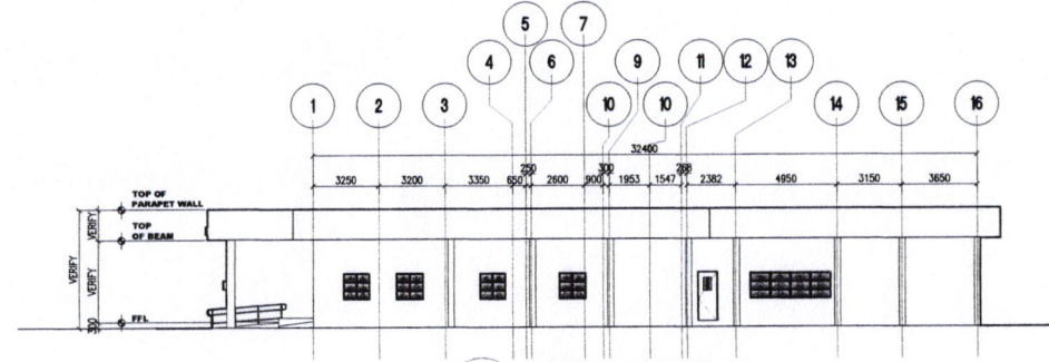
3 RIGHT ELEVATION SCALE 1:300 M A2
