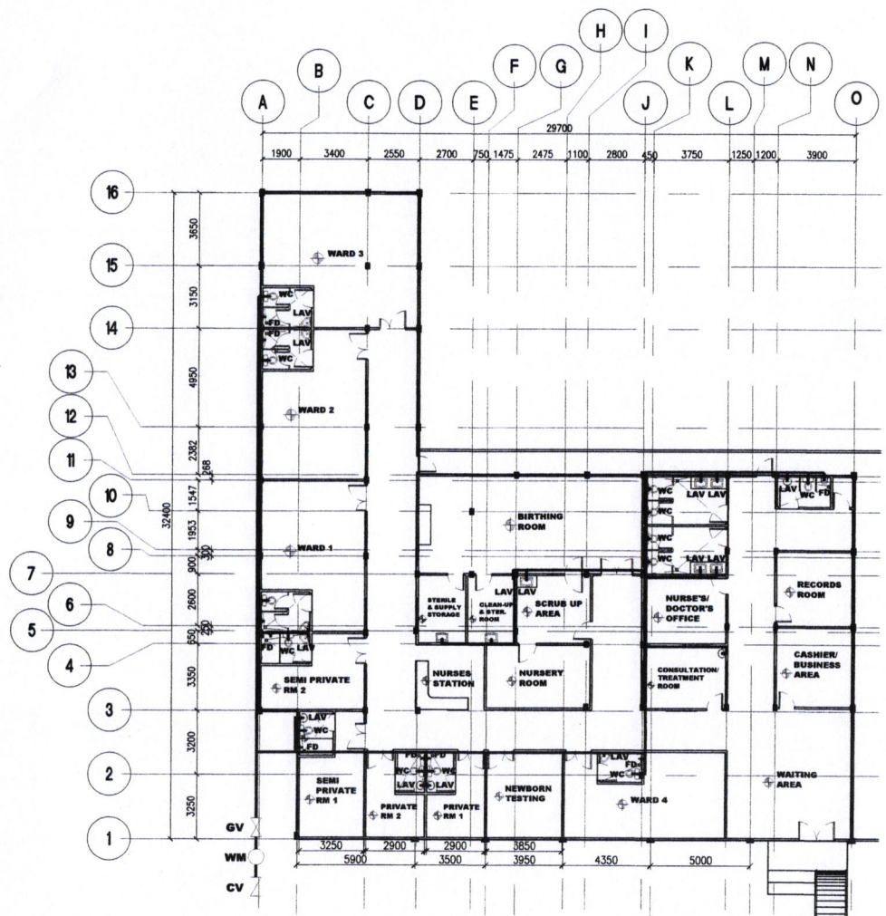
1 WATER LAYOUT PLAN P-1 SCALE 1:250M
