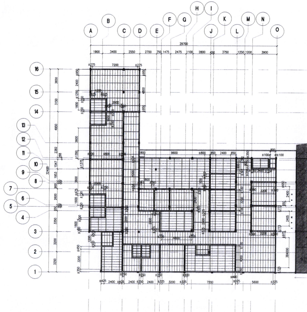
1 A6 CEILING FRAMING PLAN SCALE 1:250 M
