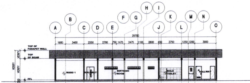
5 SECTION THRU-A SCALE 1:300 M A2
