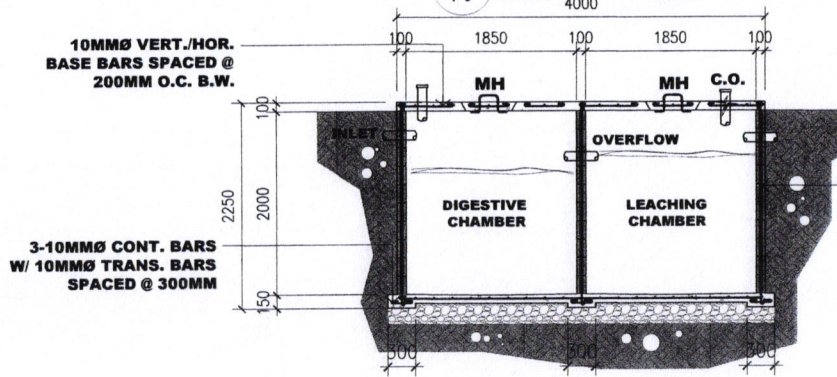
1 SEPTIC TANK SECTION SCALE 1:60M
