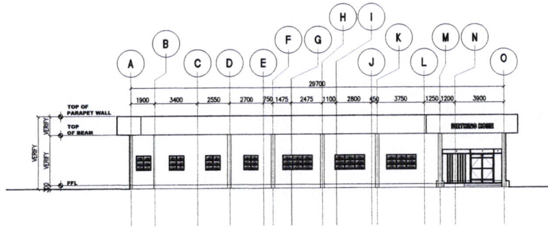
1 FRONT ELEVATION SCALE 1:300 M A2
