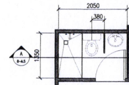
7 PRIVATE TOILET PLAN SCALE 1:16 M
