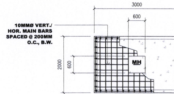
3 HAZMAT PLAN SCALE 1:60M
