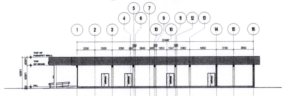
6 SECTION THRU-B SCALE 1:300 M A2
