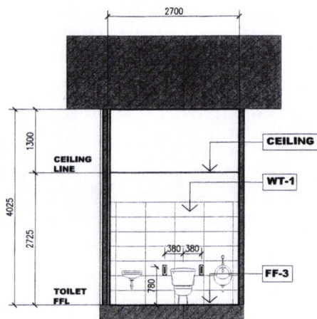
2 PWD TOILET SECTION SCALE 1:80 M
