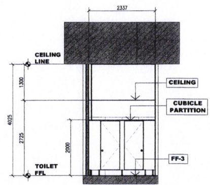
3 SECTION A SCALE 1:30 M
