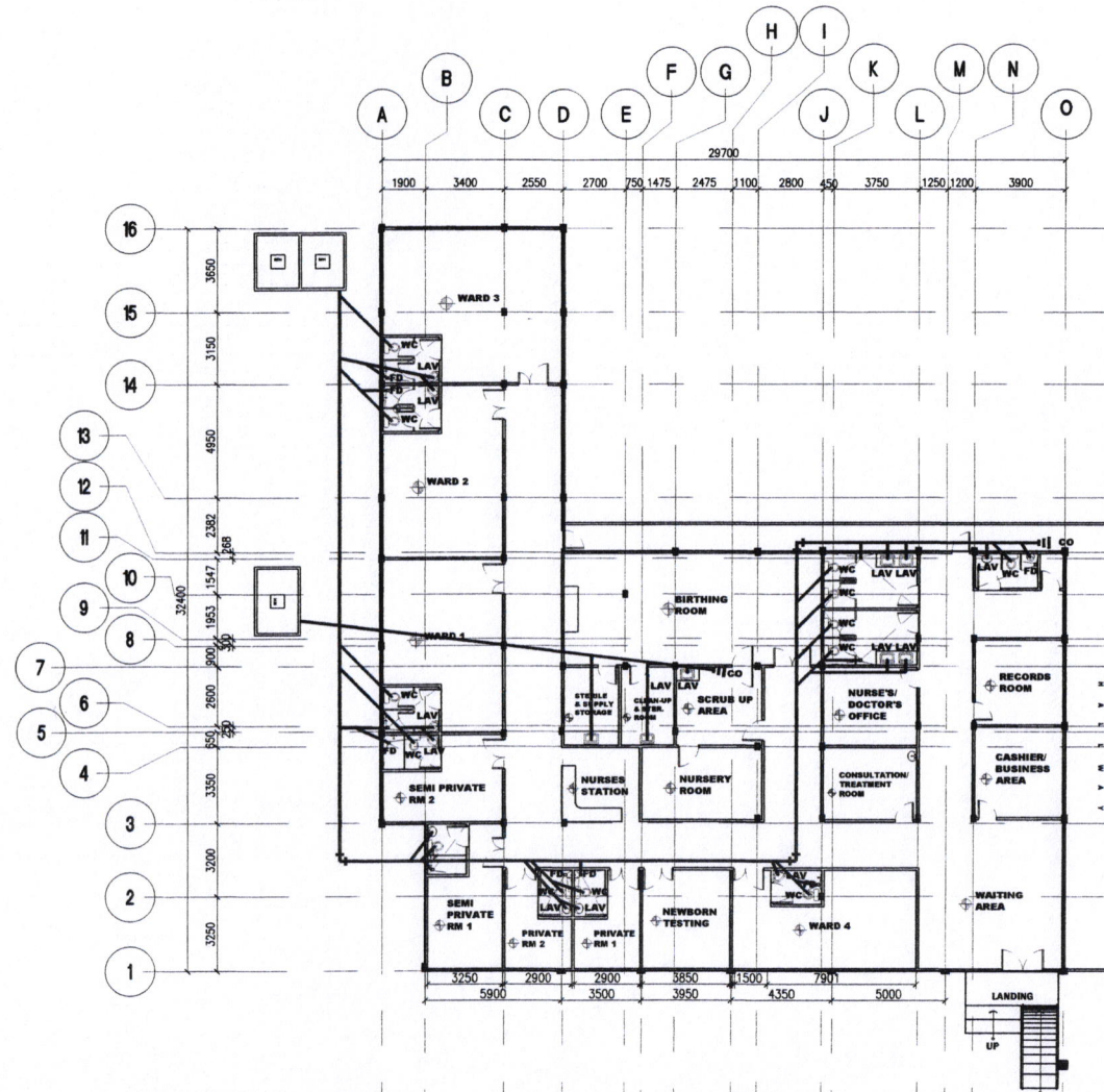
1 SANITARY LAYOUT PLAN SCALE 1:250M
