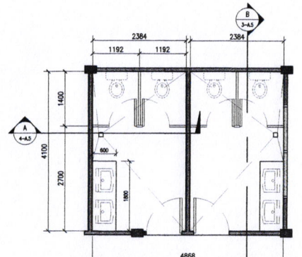
2 MALE/ FEMALE TOILET PLAN SCALE 1:30 M
