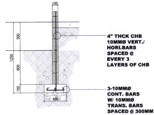
2 WF1 DETAIL SCALE 1:30 M
