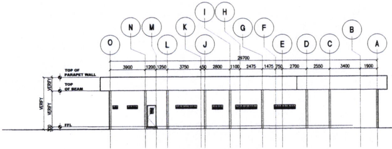
2 REAR ELEVATION SCALE 1:300 M A2
