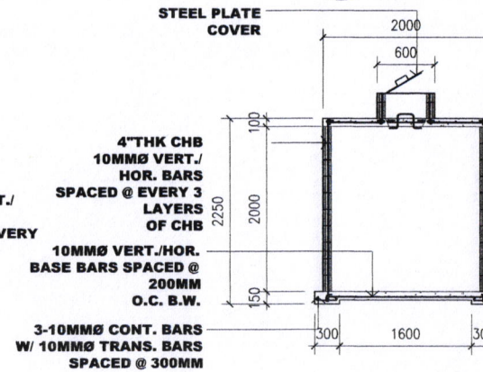
2 HAZMAT SECTION SCALE 1:60M
