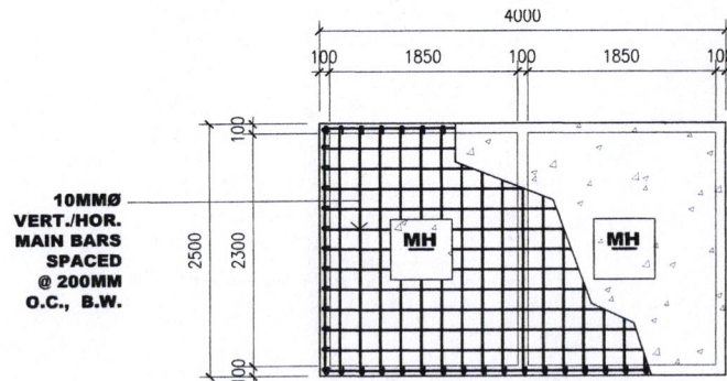
1 SEPTIC TANK PLAN SCALE 1:60M
