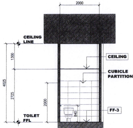
4 WARD TOILET SECTION SCALE 1:80 M
