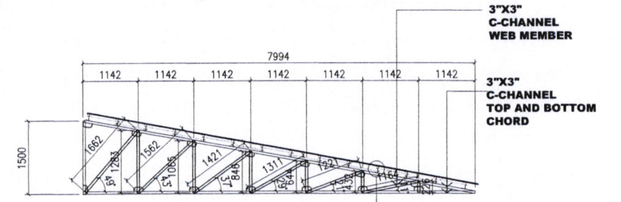
3 TRUSS DETAIL SCALE 1:180 M
