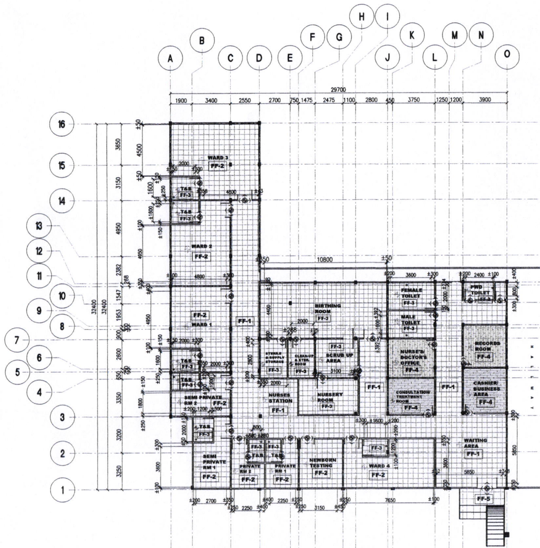
1 TILE SETTING-OUT PLAN SCALE 1:250 M
