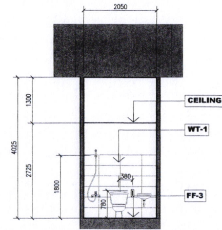
8 PRIVATE TOILET SECTION SCALE 1:80 M
