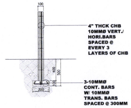
3 WF2 DETAIL SCALE 1:30 M
