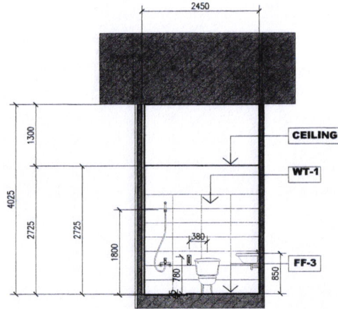
6 SEMI-PRIV. TOILET SECTION SCALE 1:80 M
