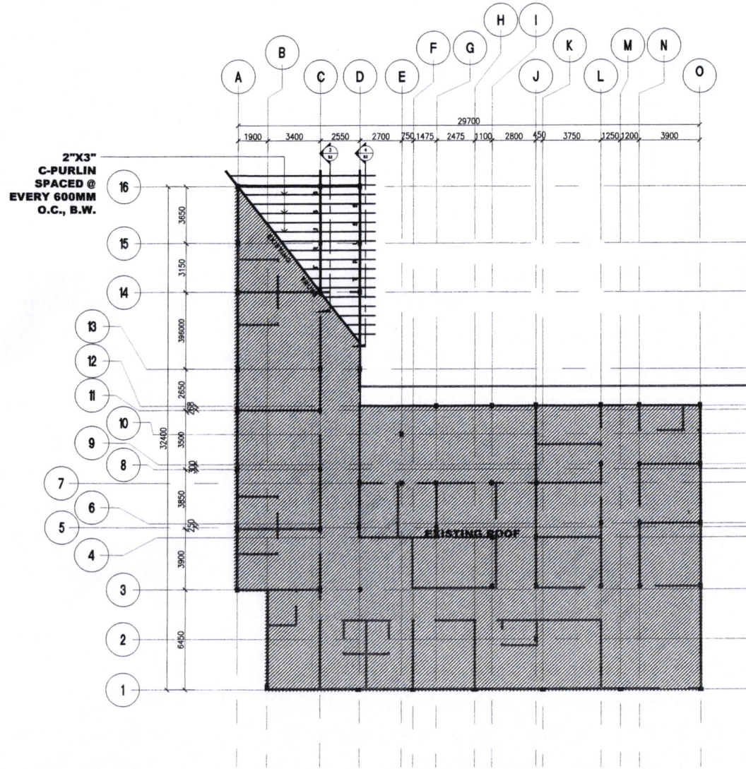
1 FOUNDATION PLAN SCALE 1:1250 M
