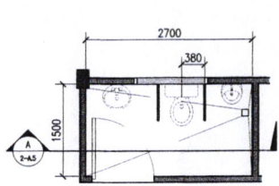
1 PWD TOILET PLAN SCALE 1:16 M
