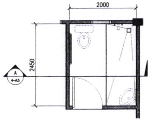
3 WARD TOILET PLAN SCALE 1:16 M
