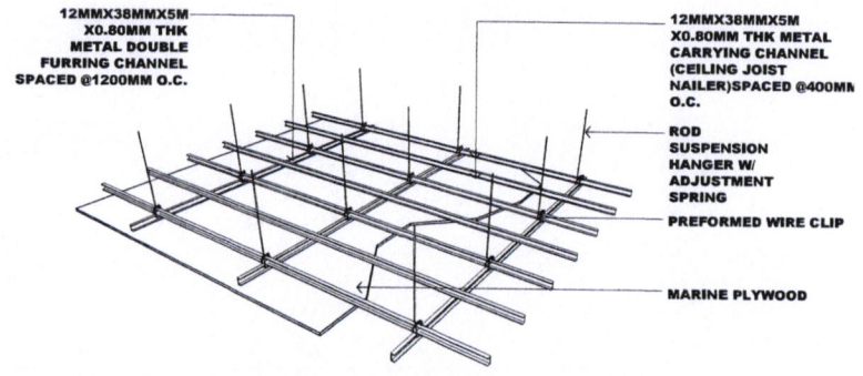
2 A6 CEILING FRAMING DETAIL SCALE NTS
