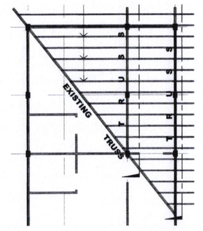
2 ROOF PLAN (BLOW-UP) SCALE 1:150 M
