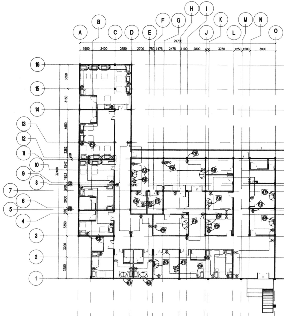
1 POWER LAYOUT PLAN SCALE 1:250 M
