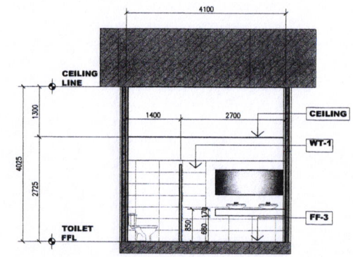
4 SECTION B SCALE 1:30 M
