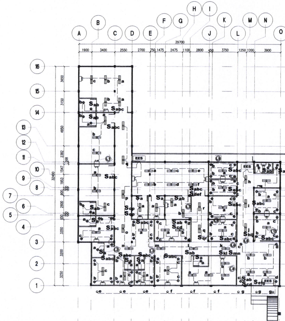
1 LIGHTING LAYOUT PLAN E1 SCALE 1:250 M
