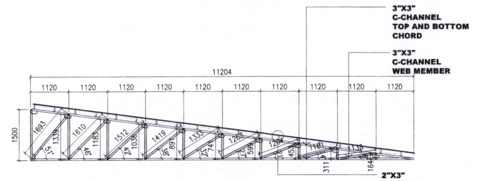
3 TRUSS DETAIL SCALE 1:180 M
