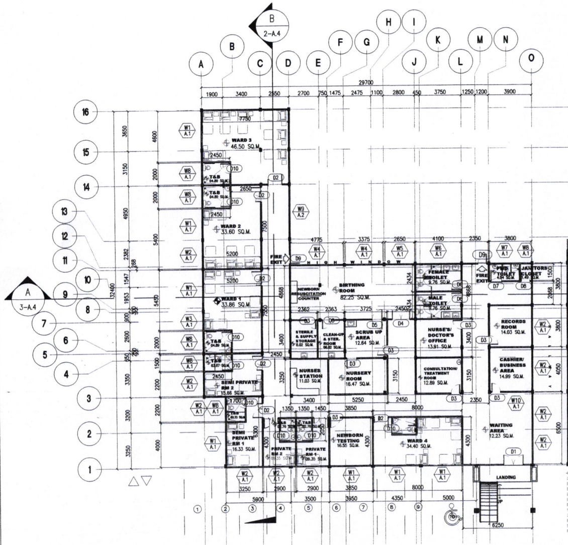
1 FLOOR PLAN SCALE 1:250 M
