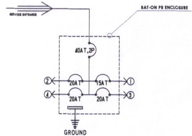
SINGLE LINE DIAGRAM AD-00 SCALE N.T.S.
