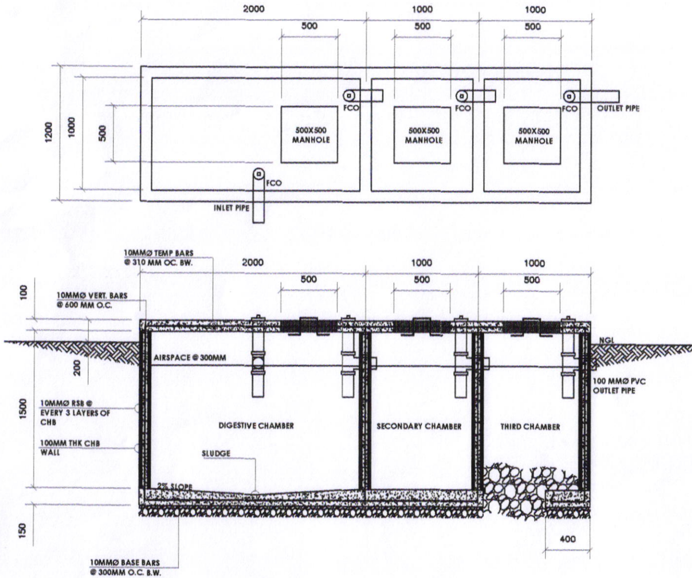
SEPTIC VAULT PLAN & SECTION AD-00 SCALE N.T.S.
