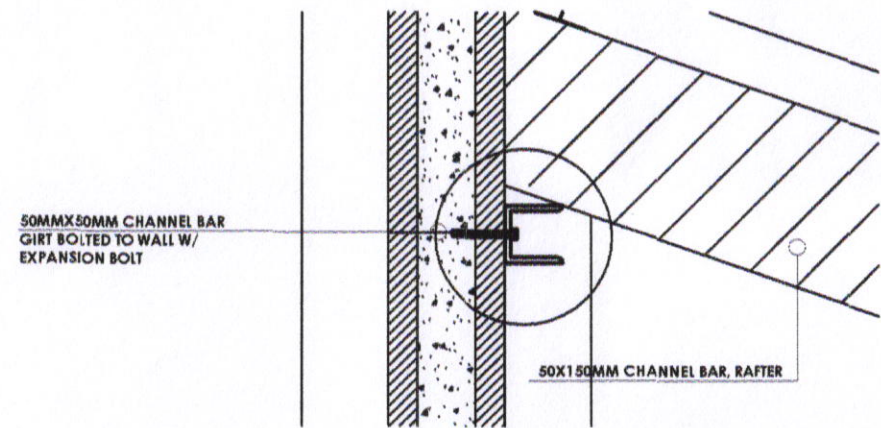
TYPICAL RAFTER DESIGN AD-00 SCALE N.T.S.
