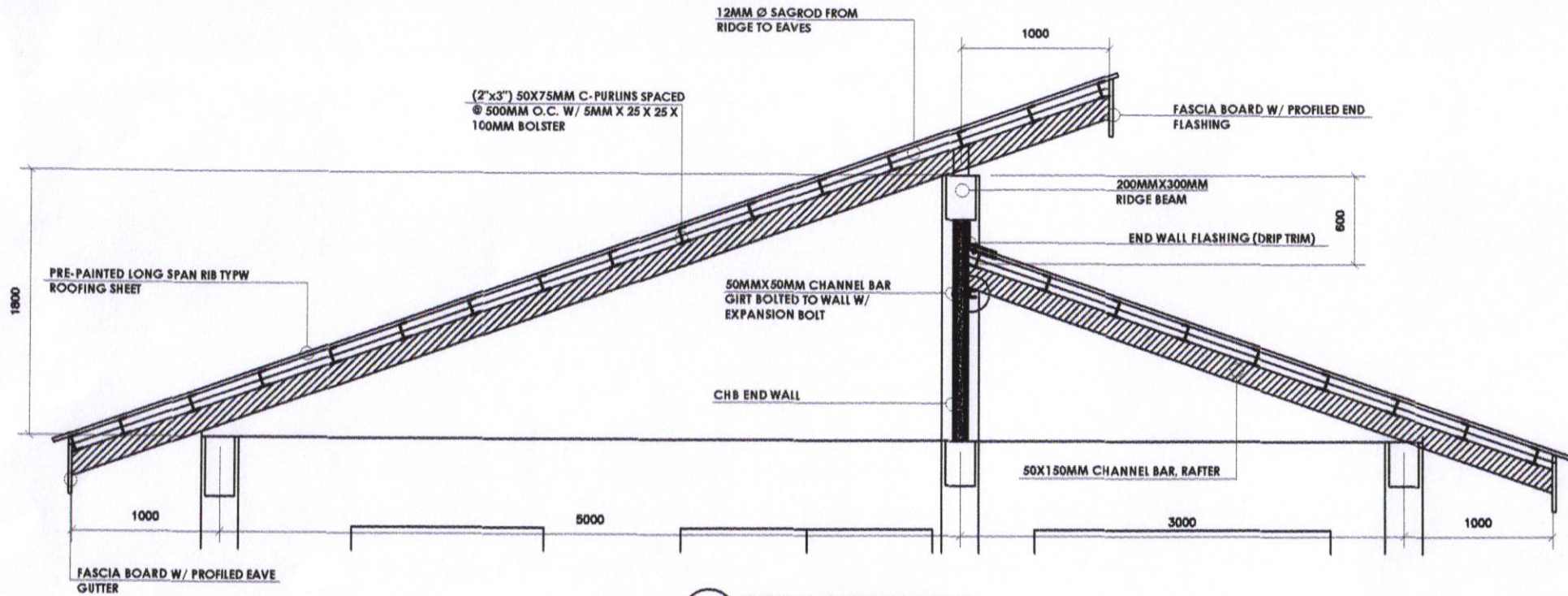
TYPICAL RAFTER DESIGN AD-00 SCALE N.T.S.
