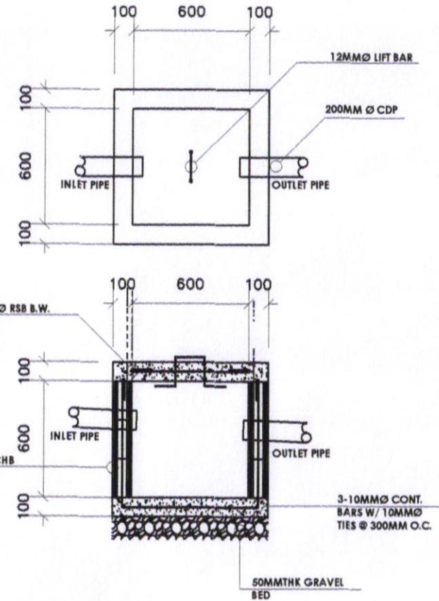
CATCH BASIN PLAN & SECTION AD-00 SCALE N.T.S.
