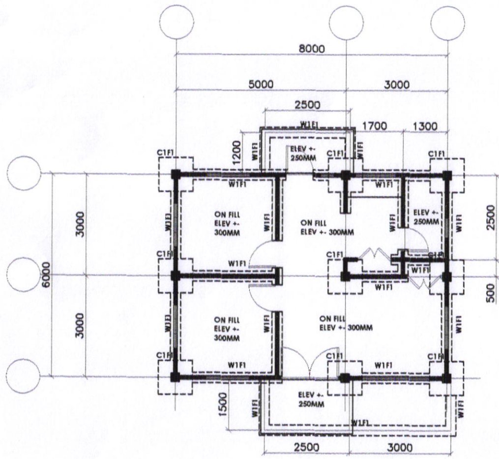
FOUNDATION PLAN AD-00 SCALE N.T.S.
