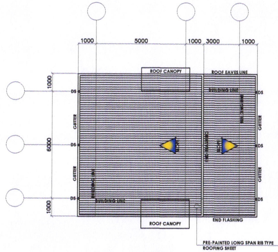
ROOF PLAN/ STORM WATER LAYOUT AD-00 SCALE N.T.S.
