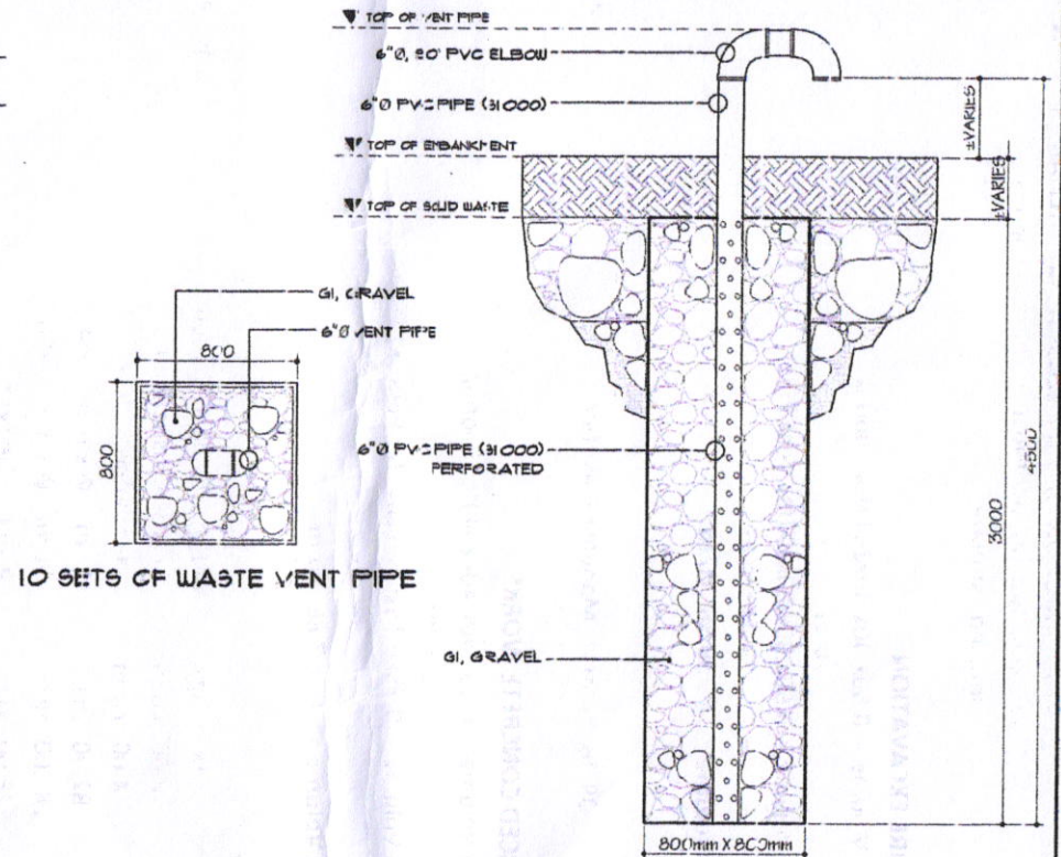
10 SETS OF WASTE VENT PIPE
