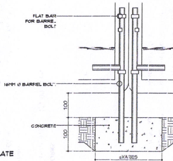
BARREL BOLT
