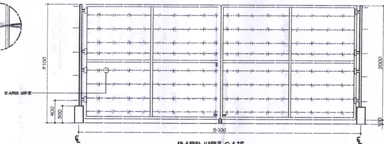
BARB WIRE GATE
