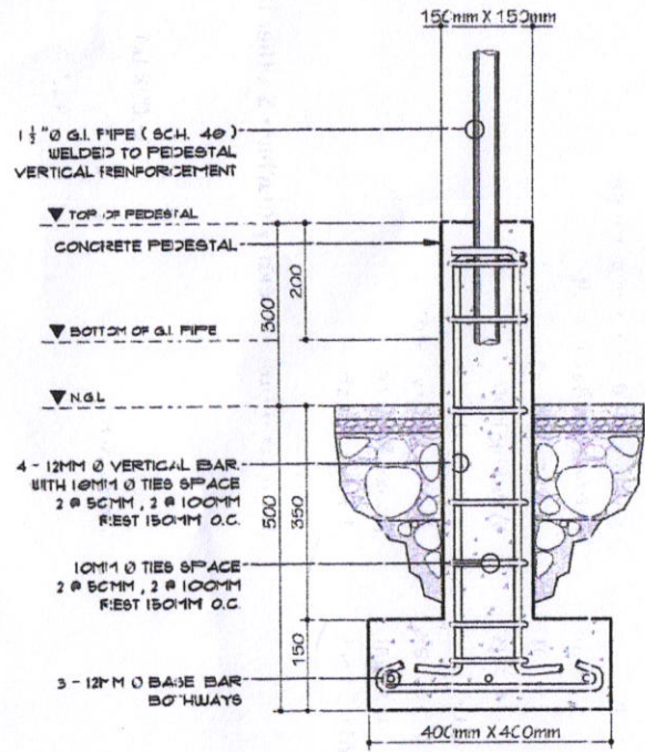
PEDESTAL DETAIL @ FENCE AND GATE
