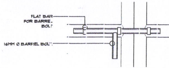
BARREL BOLT
