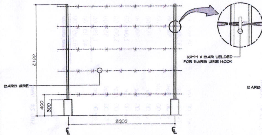
BARB WIRE FENCE ELEVATION LENGTH (L) = 418 METERS
