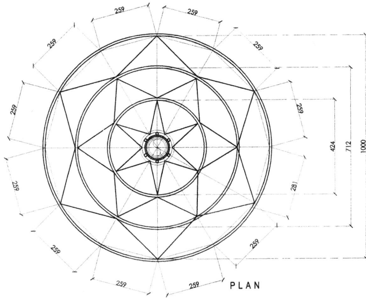
PLAN ( TOWER LANTERN )
