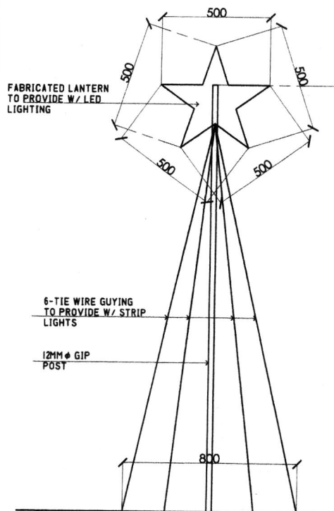
TOWER LANTERN 4 DETAIL SCALE: 1:18M.
