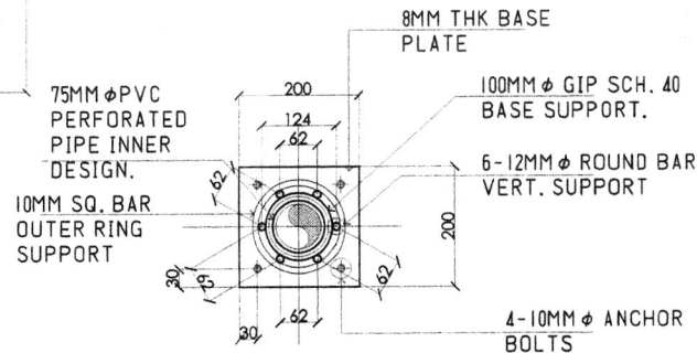
BASE PLATE PLAN
