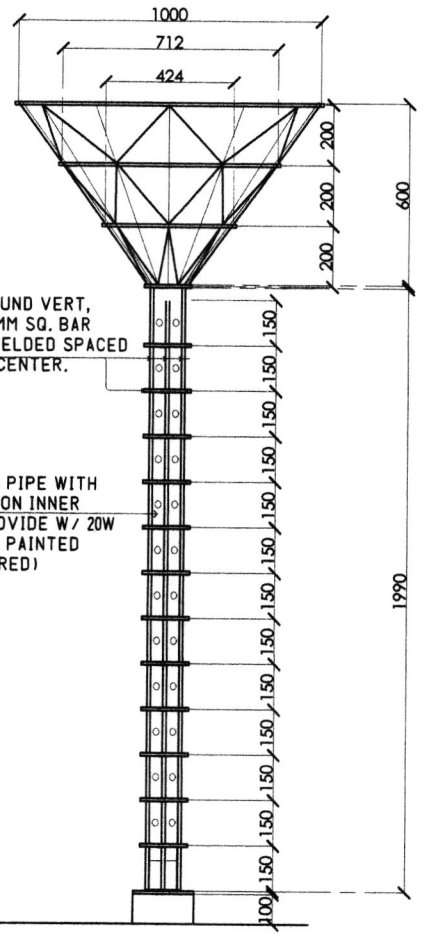
TOWER LANTERN 3 DETAIL SCALE: 1:18M.
