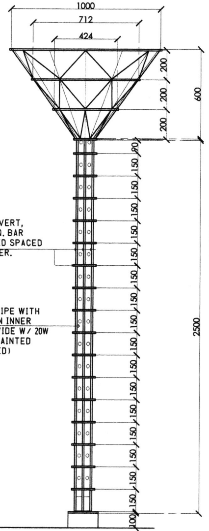
TOWER LANTERN 2 DETAIL SCALE: 1:18M.
