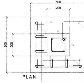
PEDESTAL/FOOTING DETAIL
