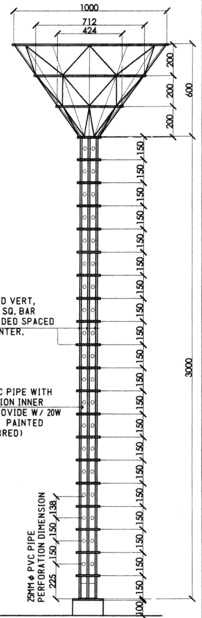
TOWER LANTERN 1 DETAIL SCALE: 1:18M.
