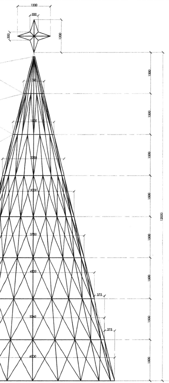
SECTIONAL ELEVATION
