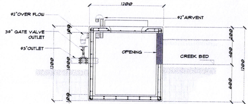
SECTION
