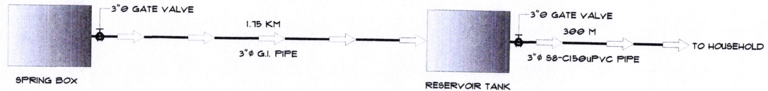
WATER SYSTEM DIAGRAM (SITIO TABANUGAO)
