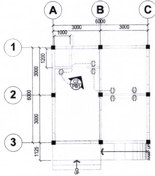
POWER LAYOUT SCALE: 1:100 MTS.
