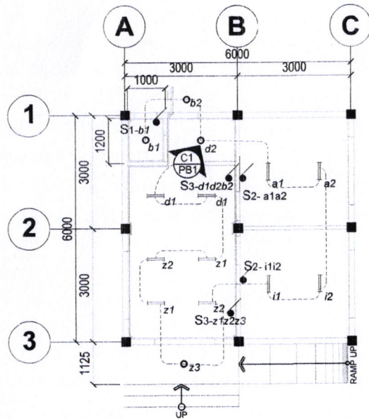
LIGHTING LAYOUT SCALE: 1:100 MTS.
