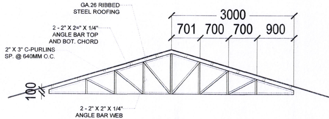
DETAIL OF FULL TRUSS SCALE: 1:40 MTS.
