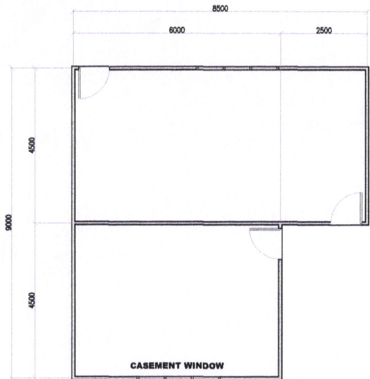
1 FLOOR PLAN (EXISTING) A-1 SCALE 1/100
