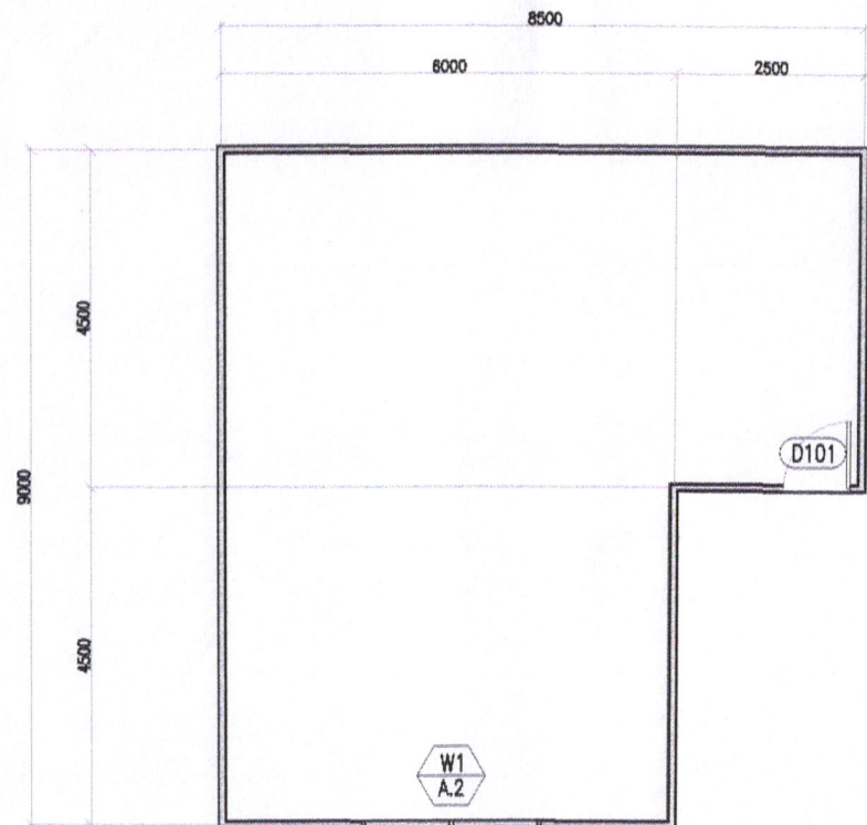
2 FLOOR PLAN (PROPOSED) A-1 SCALE 1/100
