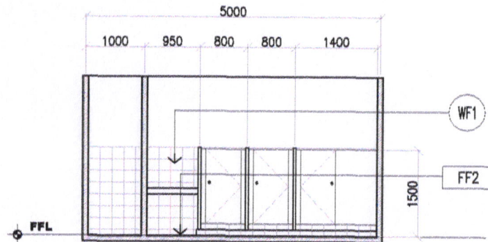
2 ELEVATION SCALE 1/100
