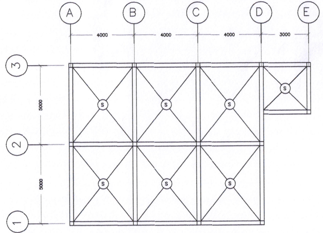
ROOF SLAB LAYOUT SCALE: 1:100MTS
