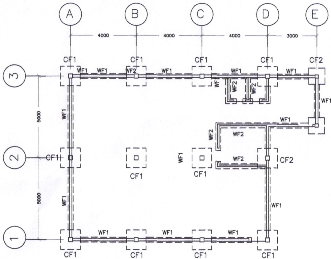
FOUNDATION PLAN SCALE: 1:100MTS
