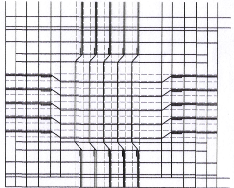
TWO-WAY SLAB DET. SCALE: 1:50MTS
