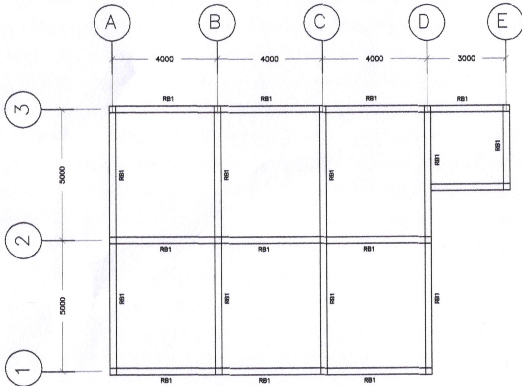
ROOF BEAM LAYOUT SCALE: 1:100MTS
