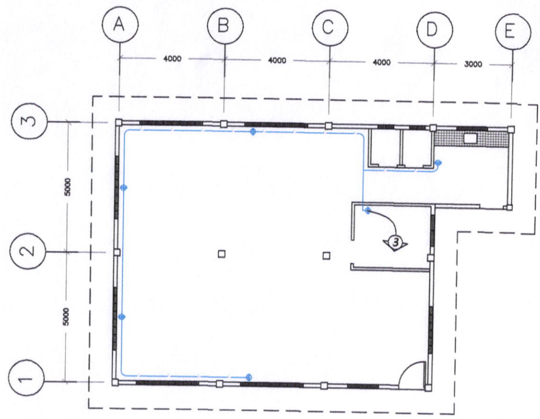
○ POWER LAYOUT SCALE: 1:100MTS
