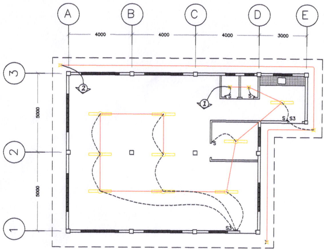
○ LIGHTING LAYOUT SCALE: 1:100MTS
