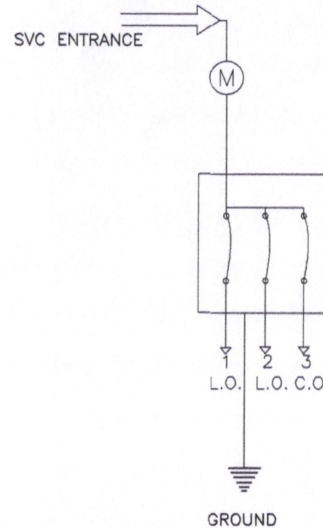
RISER DIAGRAM
