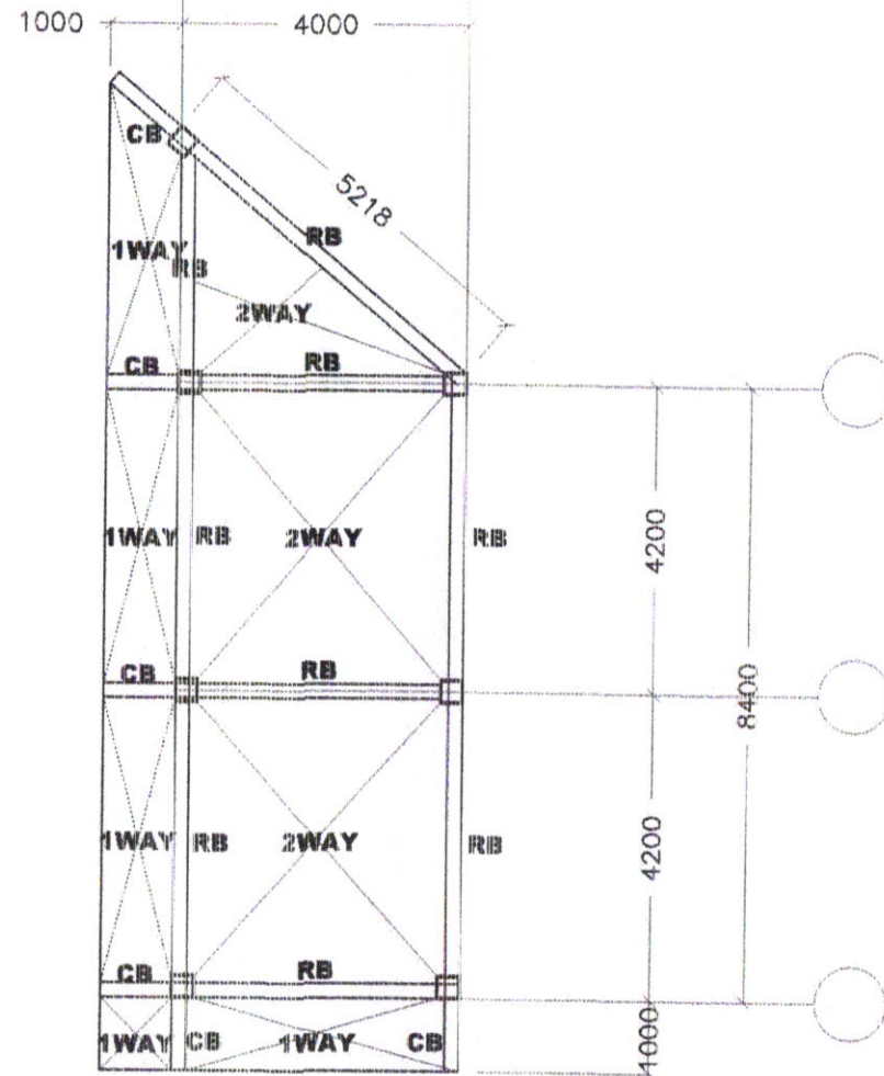
ROOF FRAMING PLAN SCALE: 1:120MTS
