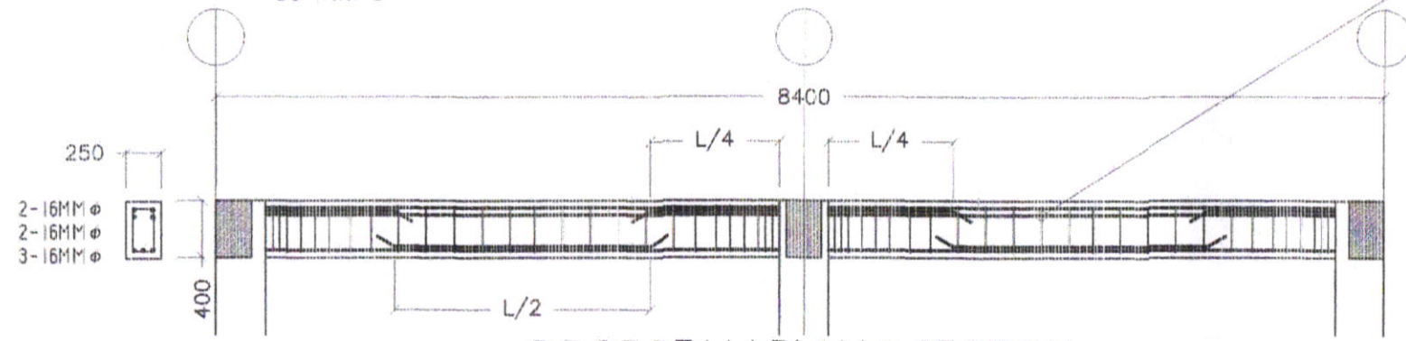
ROOF BEAM PLAN & SECTION SCALE: 1:100M
