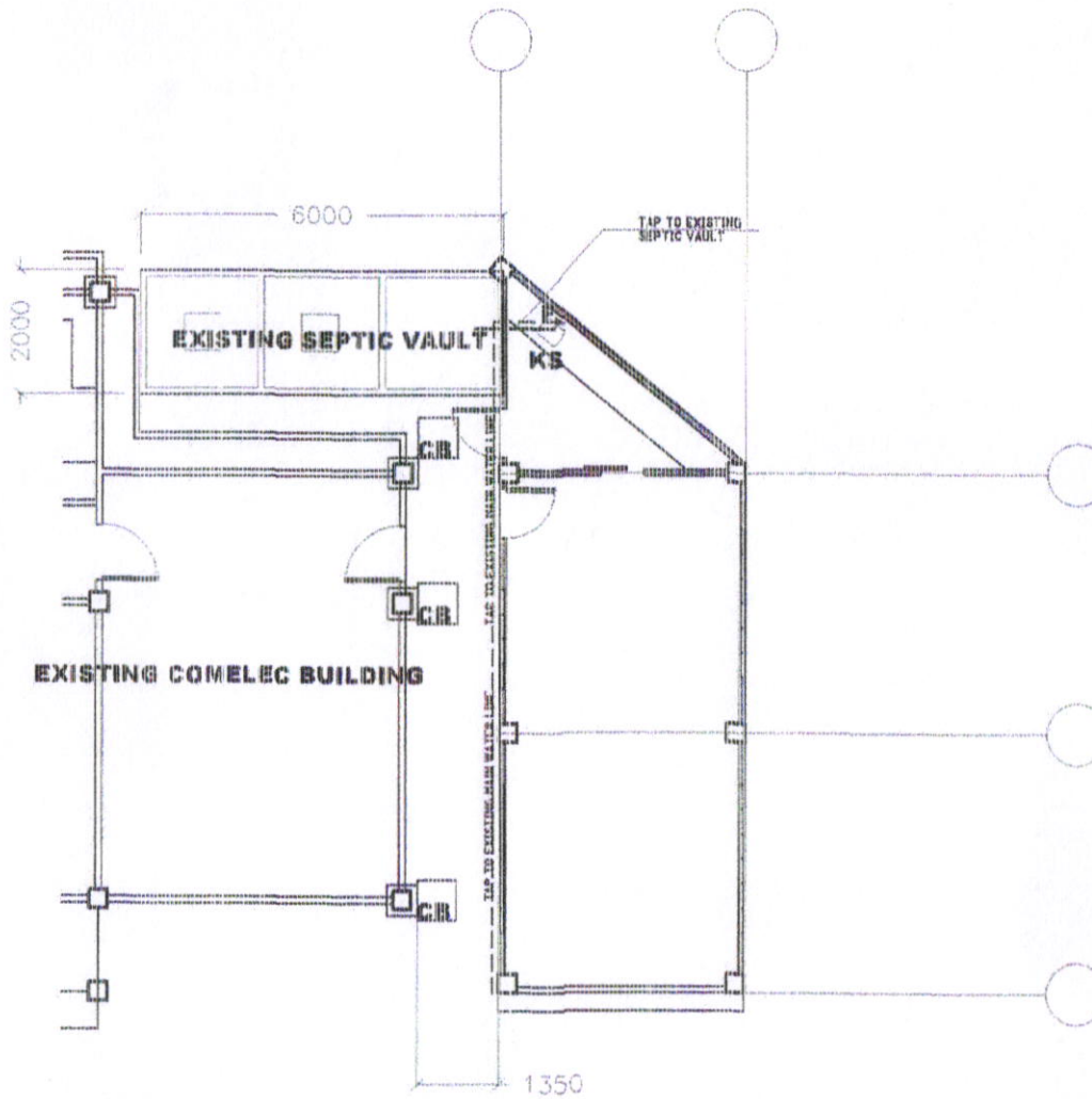
○ PLUMBING LAYOUT SCALE: 1:150M
