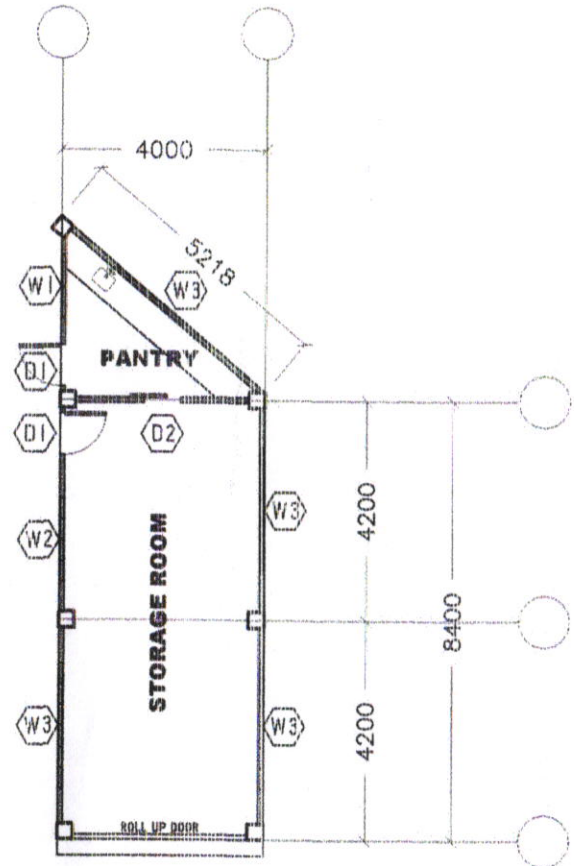
PROPOSED FLOOR PLAN SCALE: 1:20MTS
