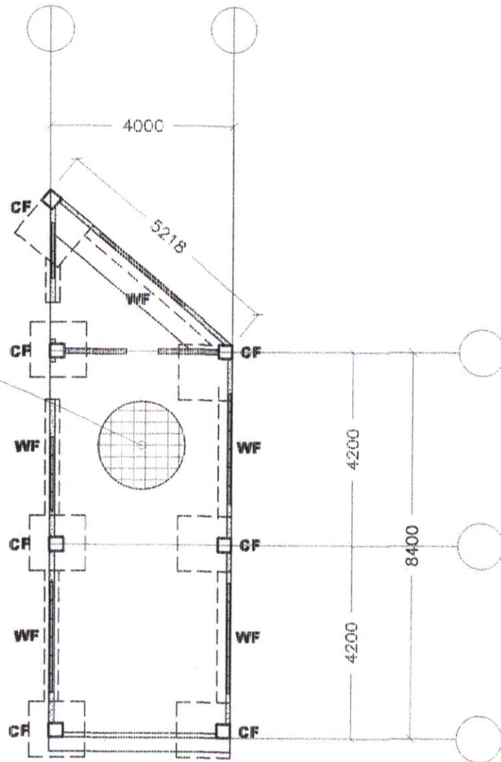
FOUNDATION PLAN SCALE: 1:120MTS
