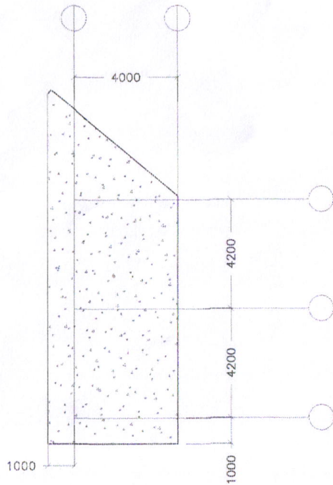
SLAB PLAN SCALE: 1:150M
