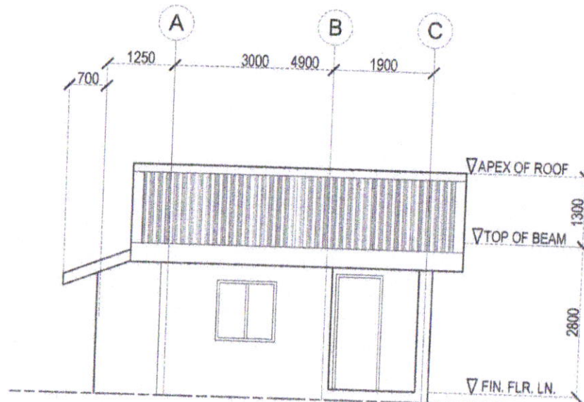
TYPICAL SIDE ELEVATION SCALE: 1:100M.
