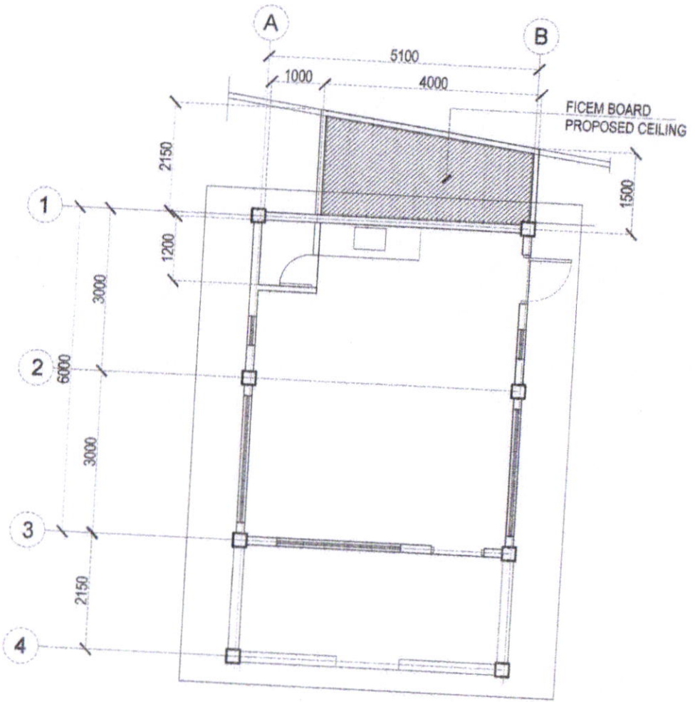
REFLECTED CEILING PLAN SCALE: 1:100M.
