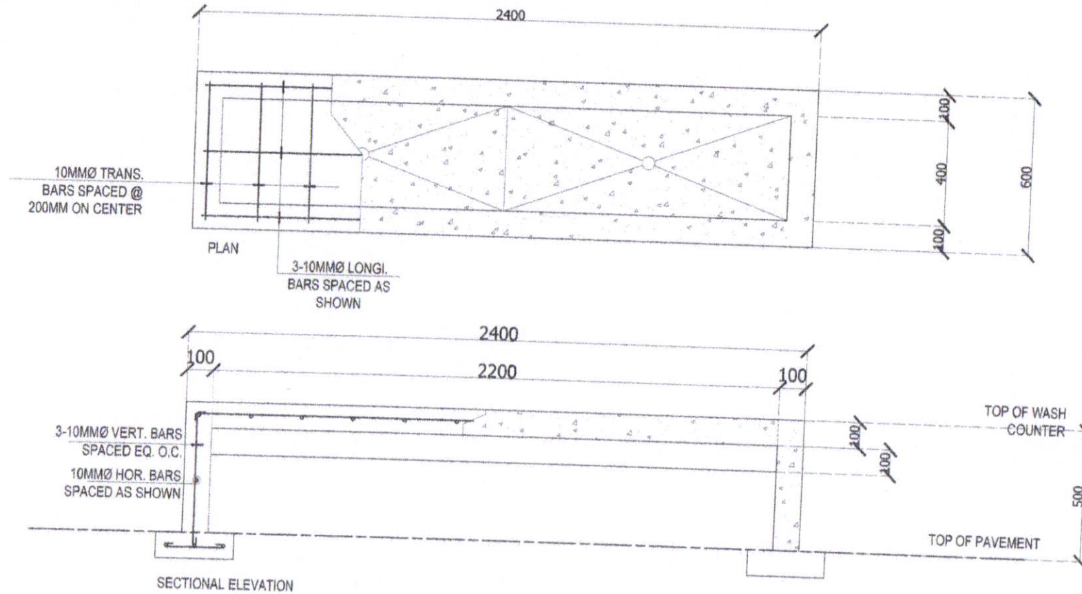
DETAIL OF HANDWASH COUNTER SCALE : 1:20M.
