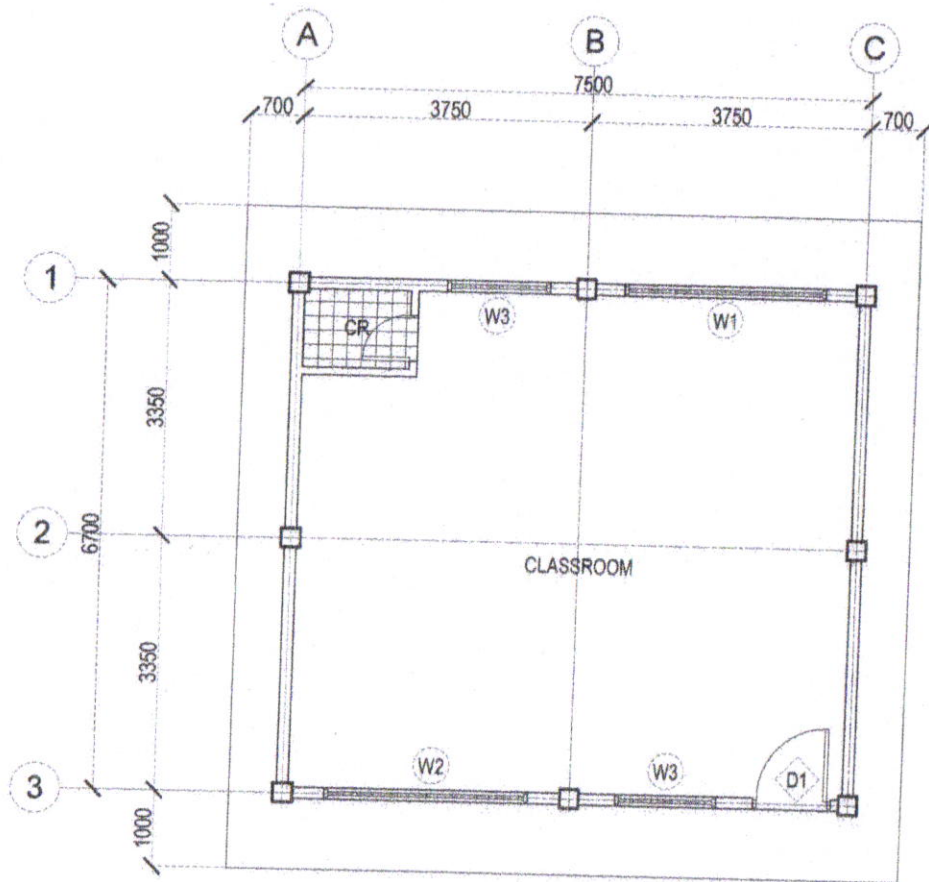
FLOOR PLAN SCALE : 1:100M.
