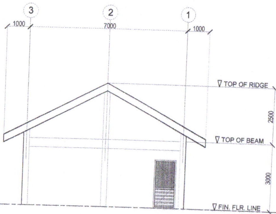
FRONT ELEVATION SCALE : 1:100M.
