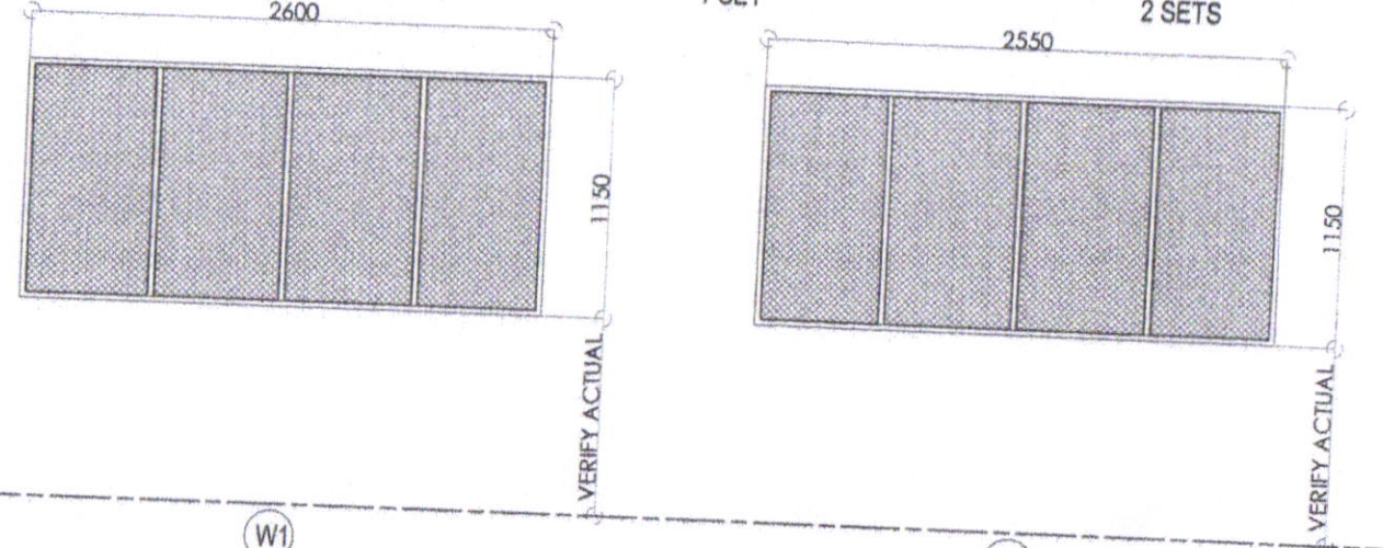
SCHEDULE OF DOORS & WINDOWS SCALE: 1:40M.
