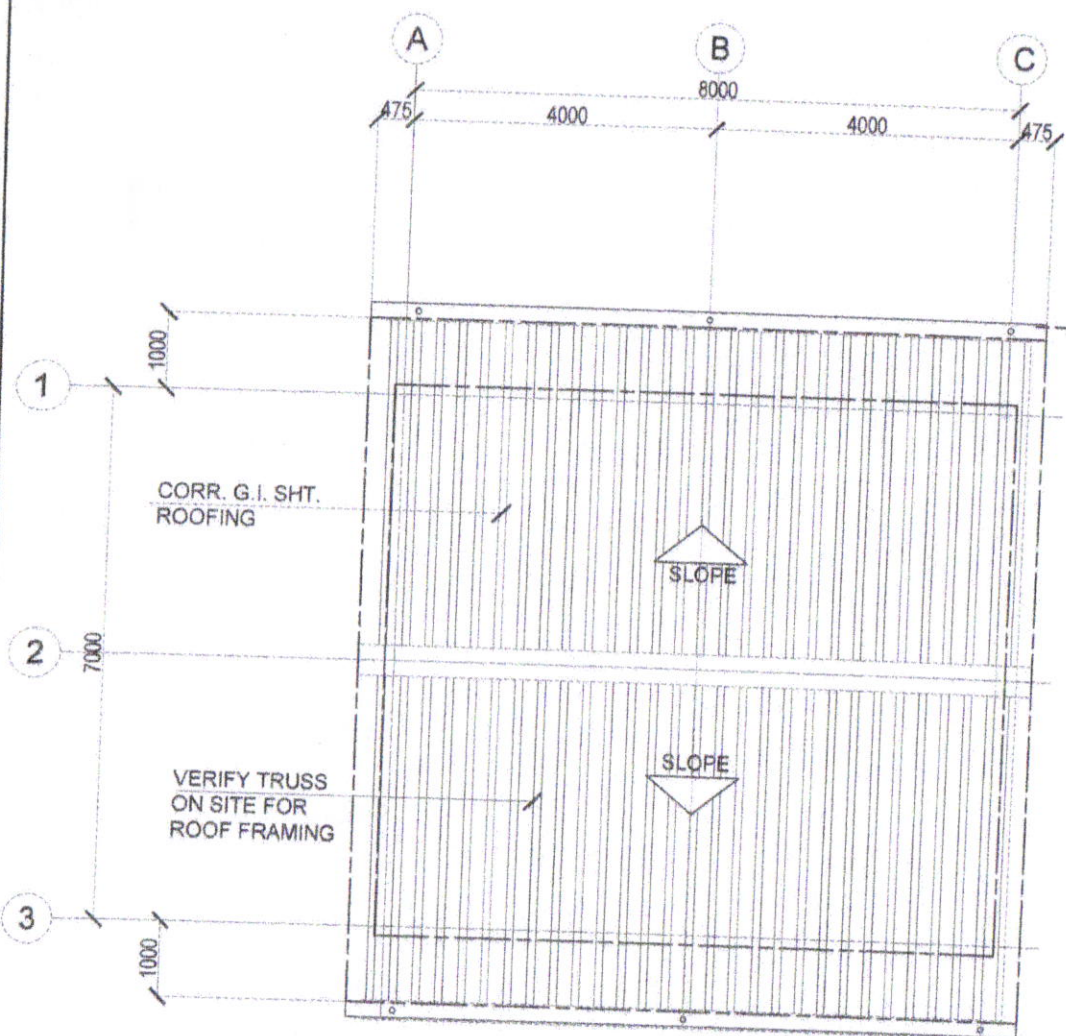
ROOF PLAN SCALE : 1:100M.
