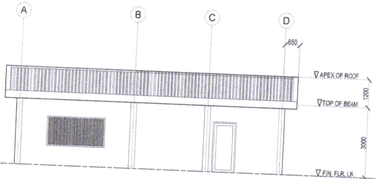
FRONT ELEVATION SCALE : 1:100M.
