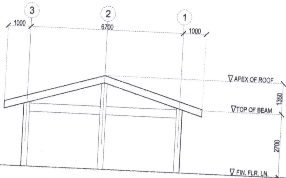
RIGHT SIDE ELEVATION SCALE : 1:100M.
