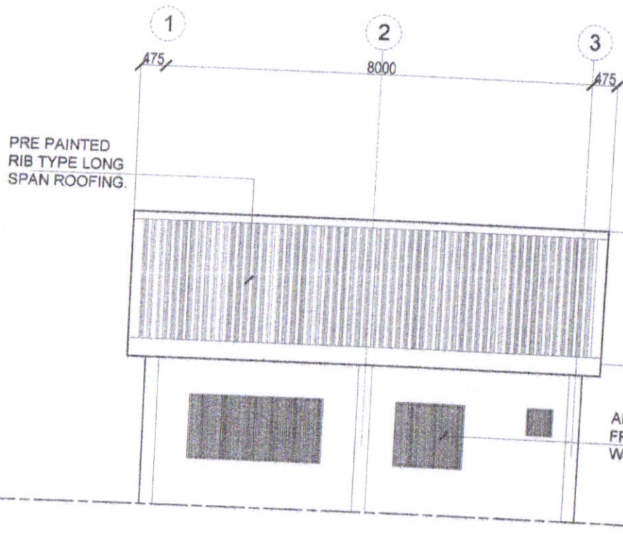
LEFT SIDE ELEVATION SCALE : 1:100M.
