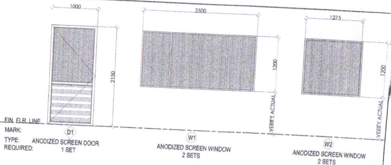
SCHEDULE OF SCREEN WINDOWS & DOORS SCALE : 1:40M.
