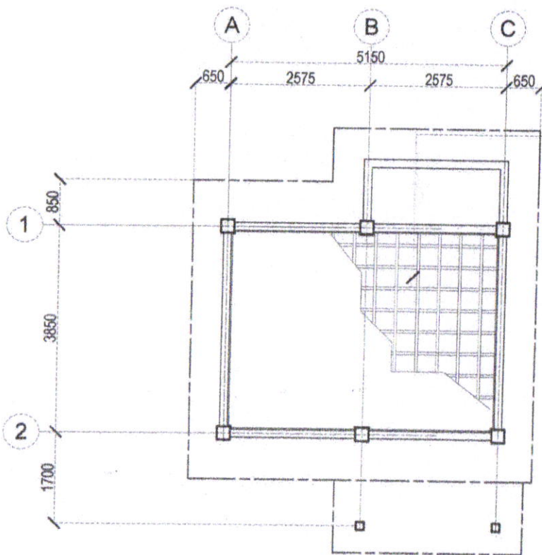
REFLECTED CEILING PLAN SCALE: 1:100M.
