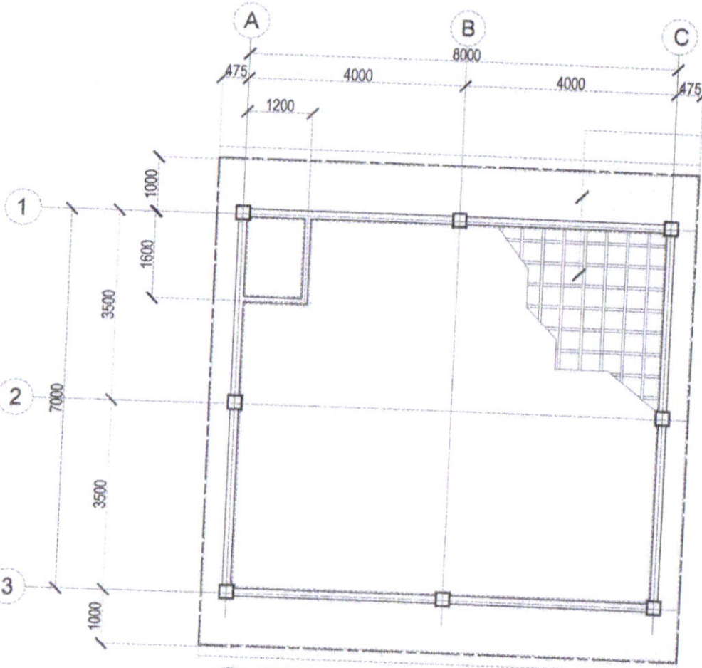
REFLECTED CEILING PLAN SCALE: 1:100M.
