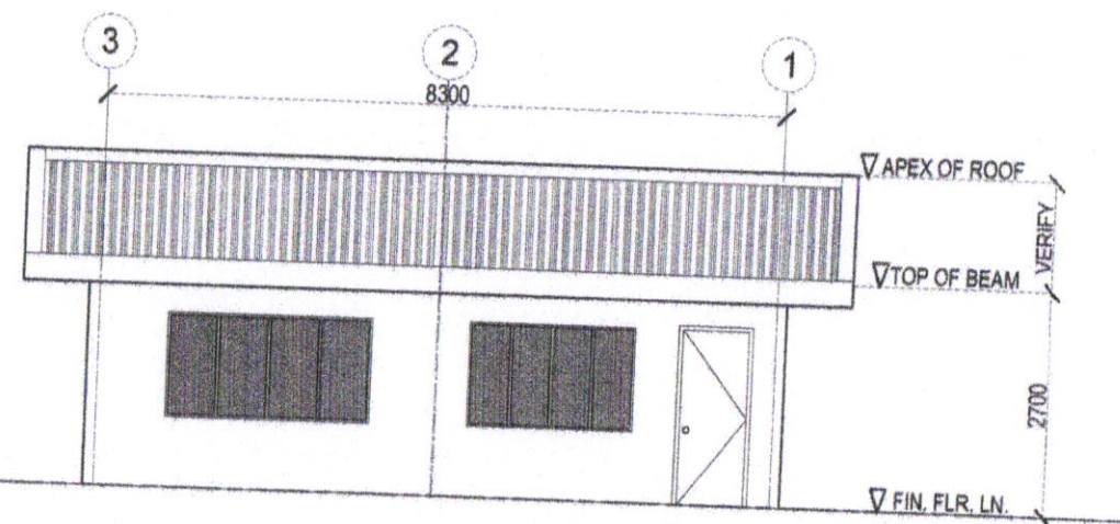
RIGHT SIDE ELEVATION SCALE : 1:100M.
