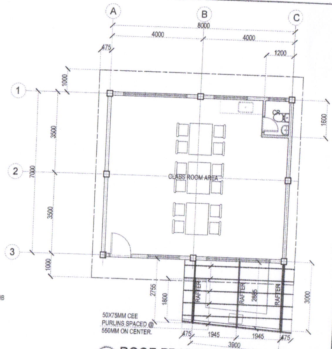
ROOF FRAMING PLAN (KITCHEN) SCALE: 1:100M.
