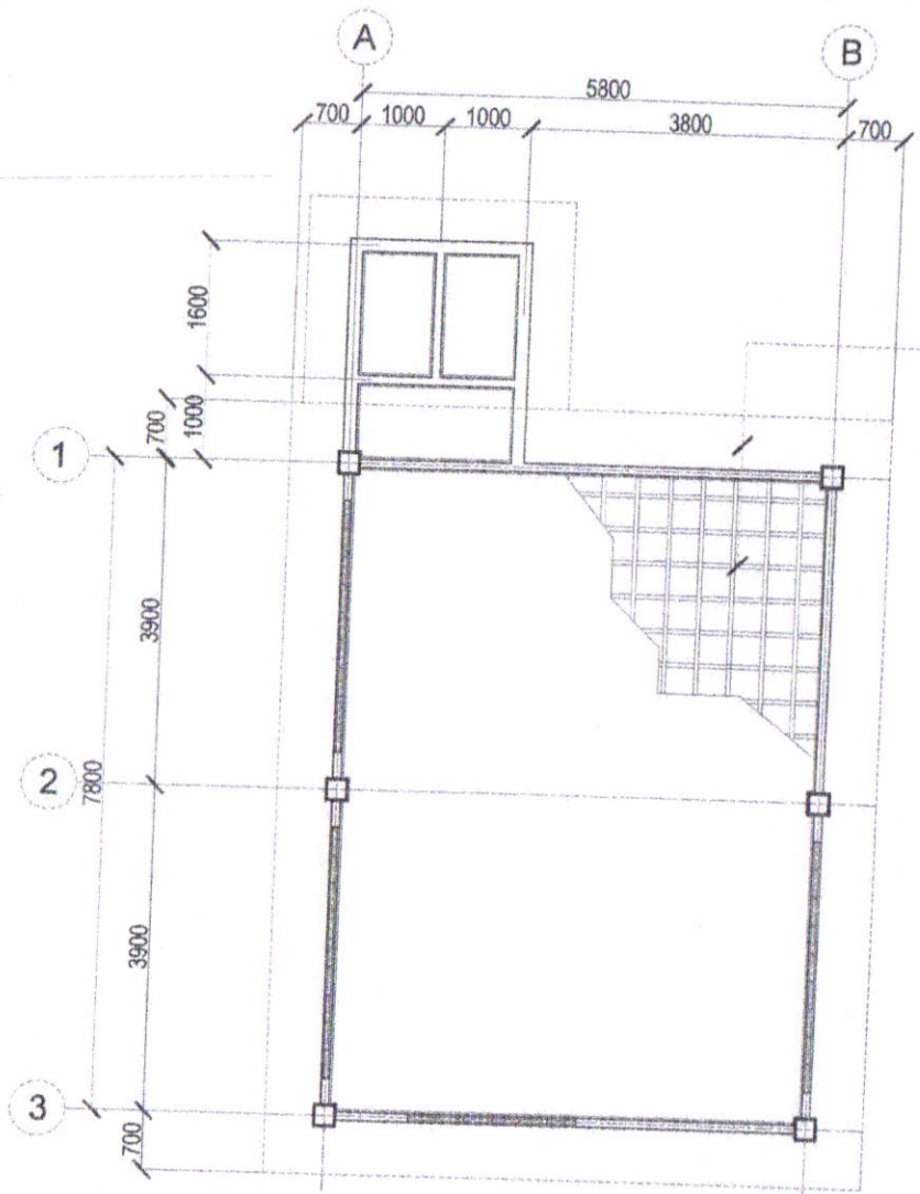
REFLECTED CEILING PLAN SCALE: 1:100M.
