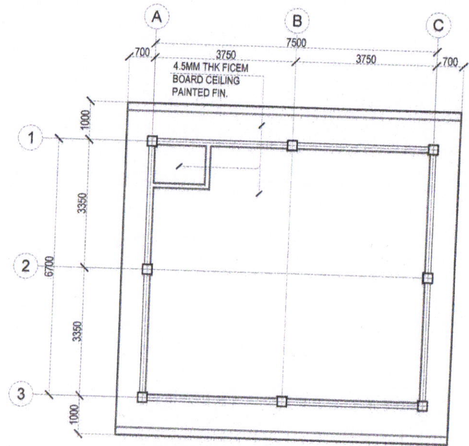
REFLECTED CEILING PLAN SCALE : 1:100M.
