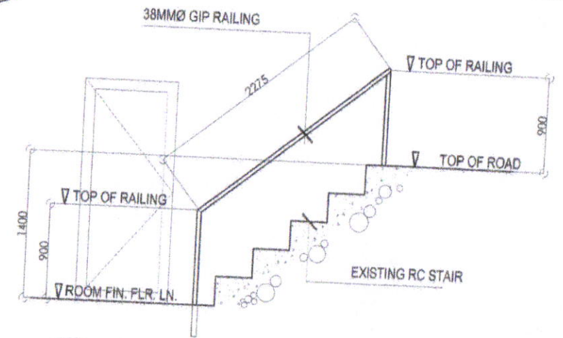
DETAIL OF RAILINGS SCALE : 1:40M.
