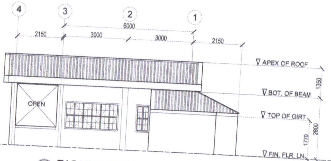
RIGHT SIDE ELEVATION SCALE : 1:100M.
