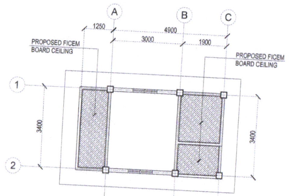
REFLECTED CEILING PLAN SCALE: 1:100M.
