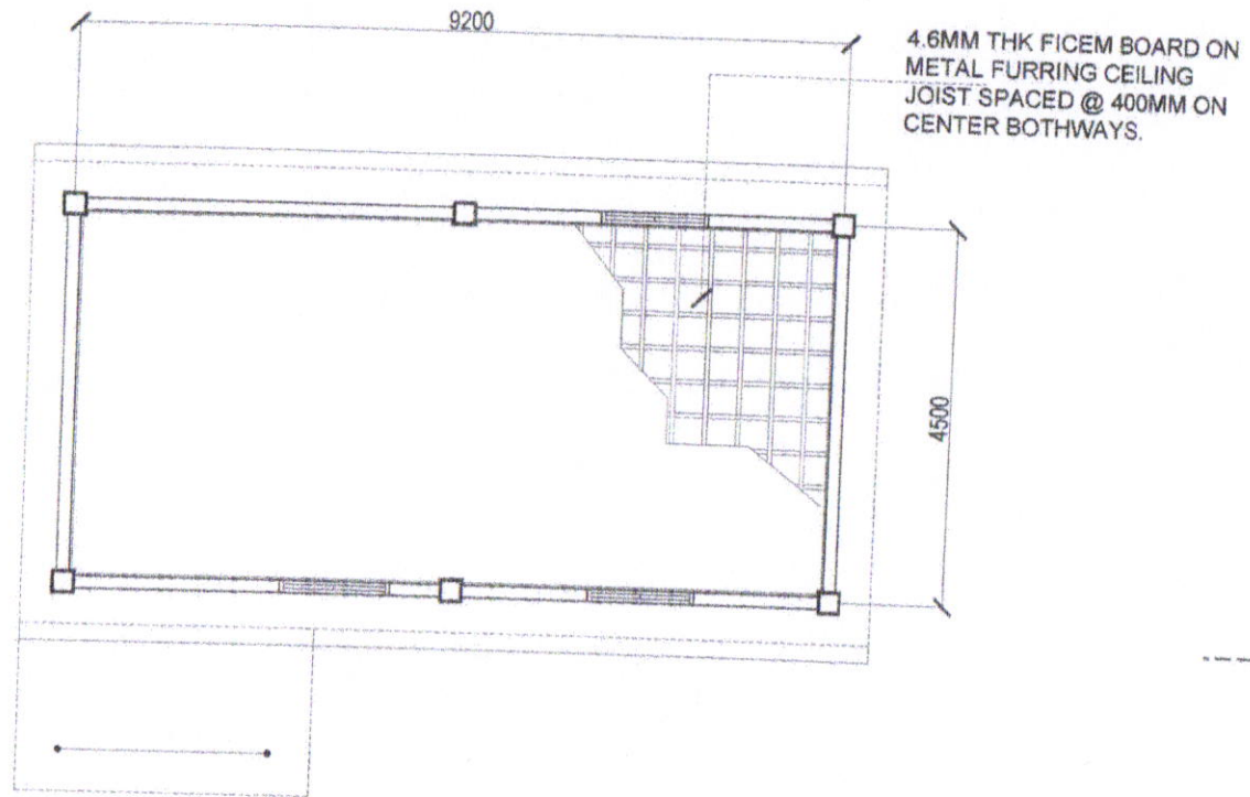
REFLECTED CEILING PLAN SCALE : 1:100M.
