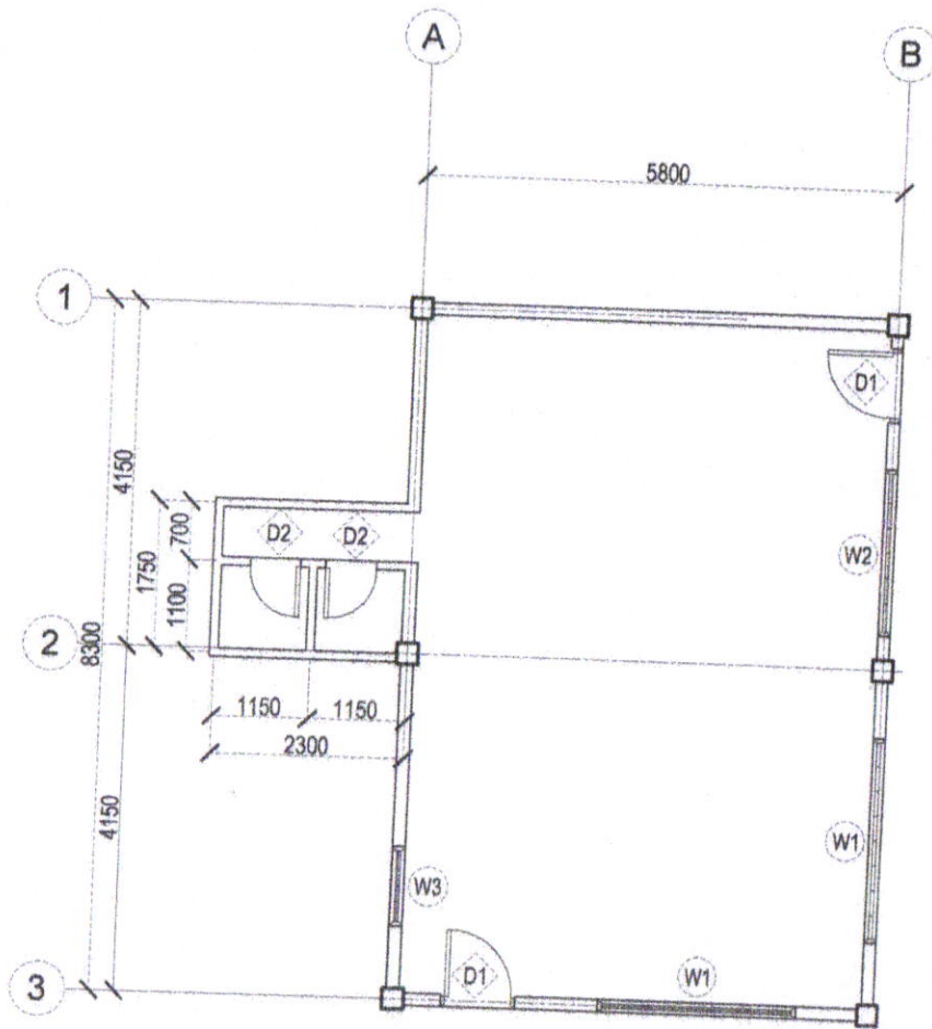
FLOOR PLAN SCALE : 1:100M.
