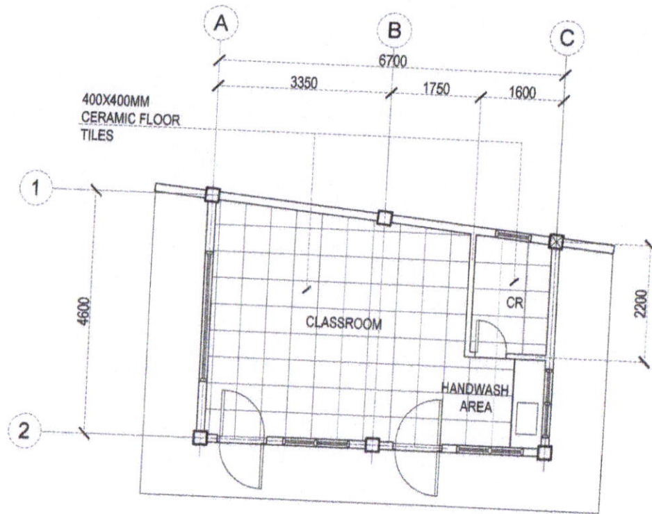
FLOOR TILES LAY OUT PLAN SCALE : 1:100M.
