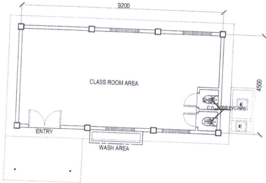
FLOOR PLAN SCALE : 1:100M.
