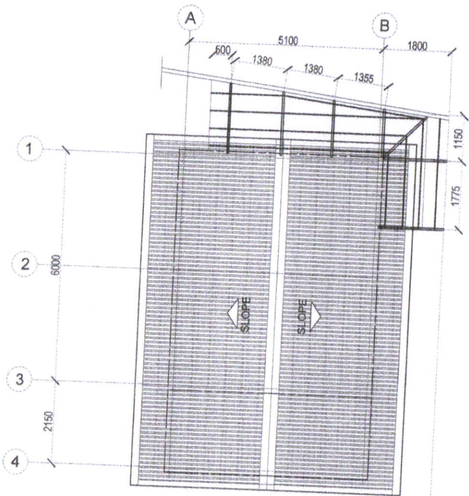
ROOF/ FRAMING PLAN SCALE : 1:100M.
