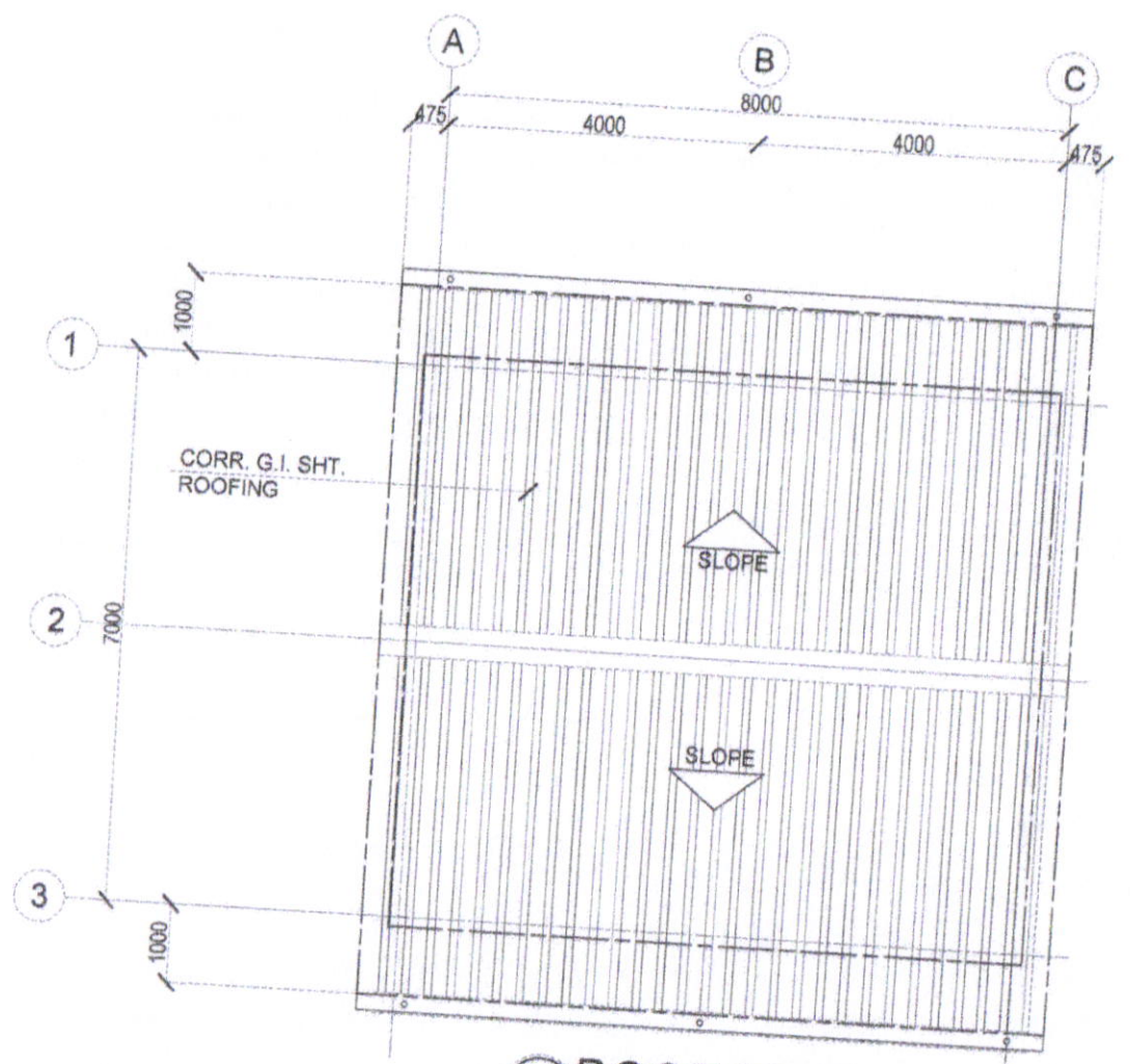
ROOF PLAN SCALE : 1:100M.
