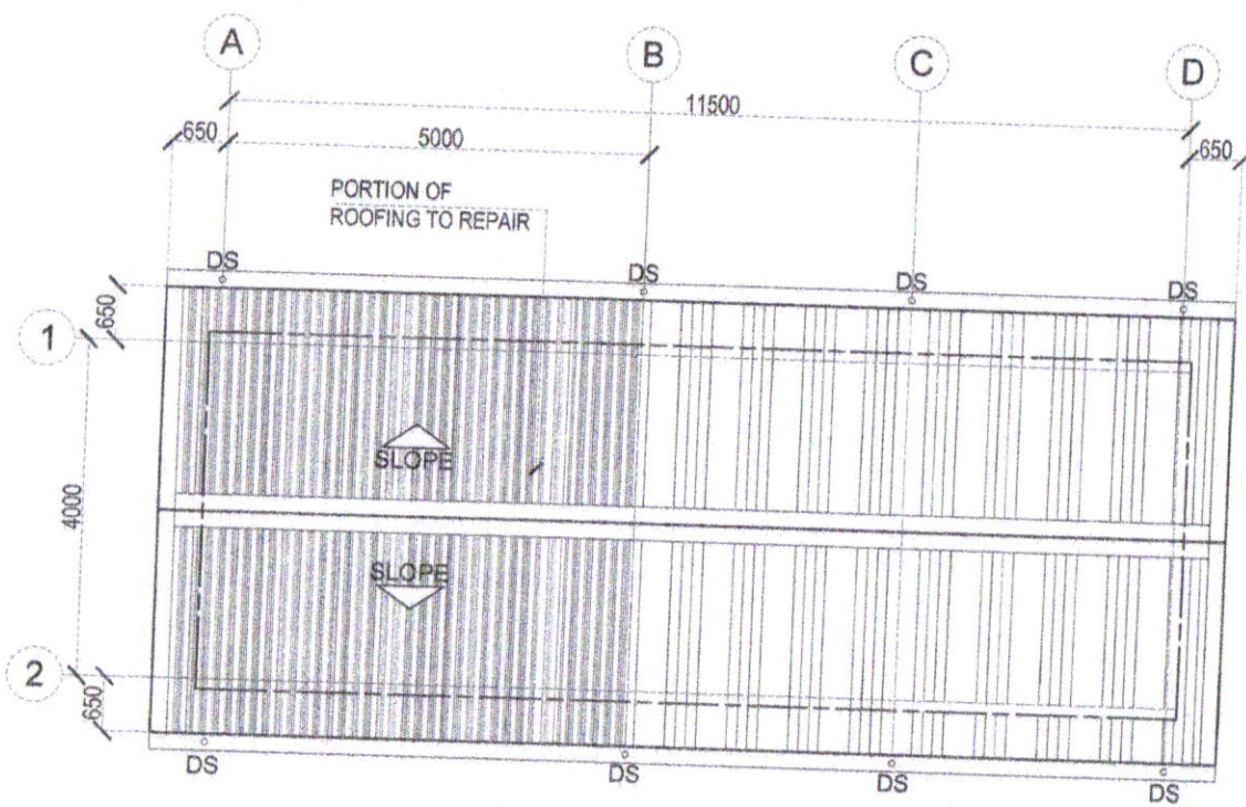
ROOF PLAN SCALE : 1:100M.
