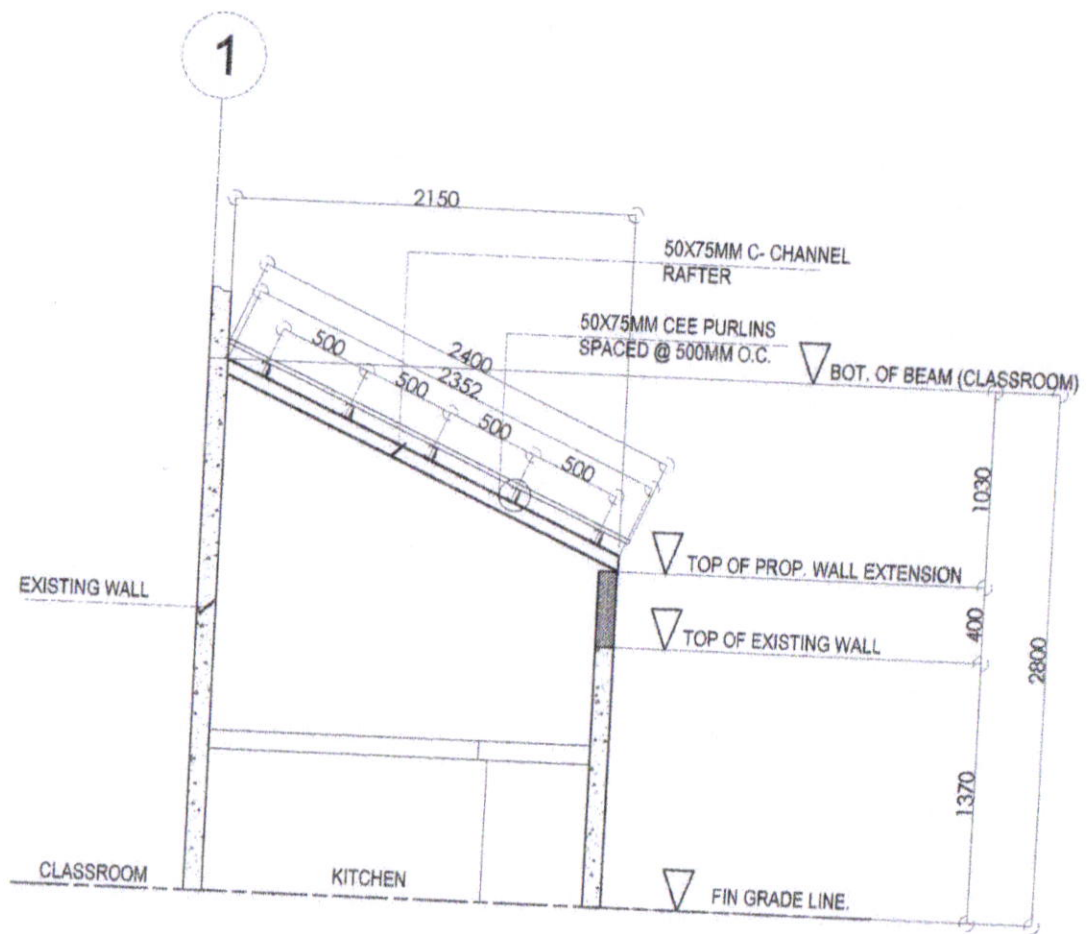
RAFTER DETAIL SCALE : 1:40M.
