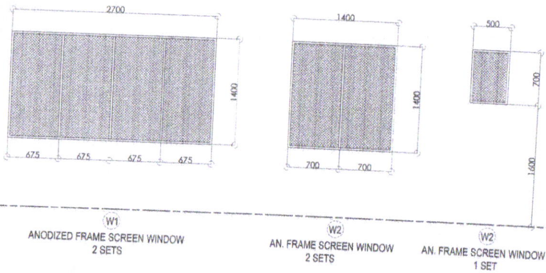
SCHEDULE OF SCREEN WINDOWS & DOORS SCALE: 1:50M.
