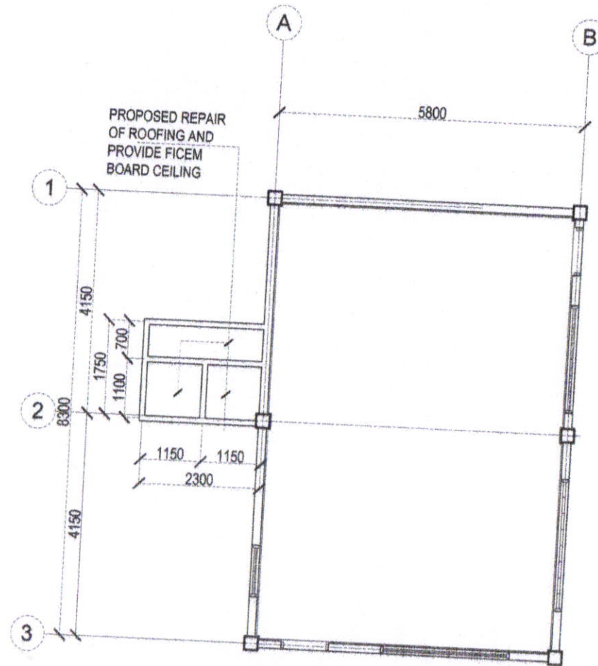
REFLECTED CEILING PLAN SCALE : 1:100M.
