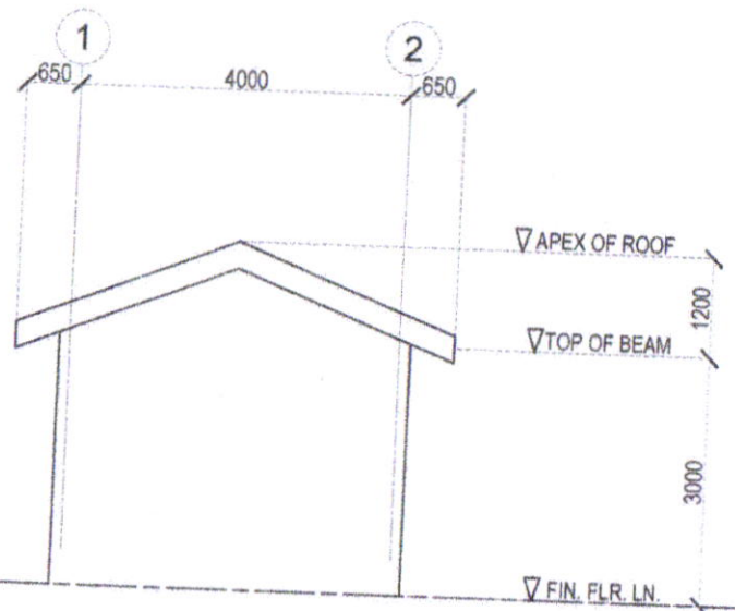
TYPICAL SIDE ELEVATION SCALE : 1:100M.
