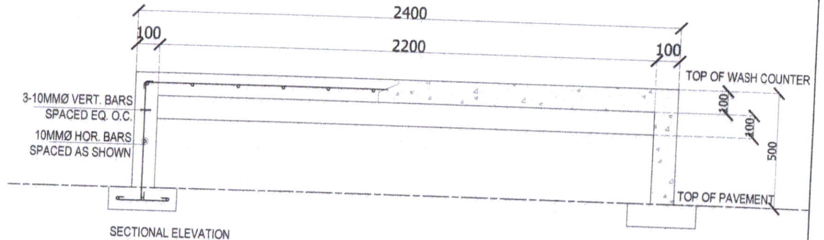
DETAIL OF HANDWASH COUNTER SCALE: 1:16M.
