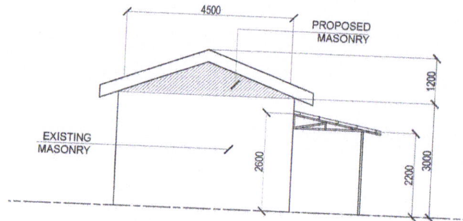
LEFT SIDE ELEVATION SCALE : 1:100M.
