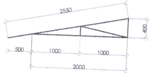
TRUSS DIAGRAM SCALE : 1:45M.
