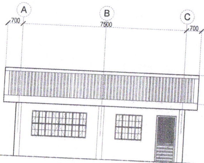
FRONT ELEVATION SCALE : 1:100M.
