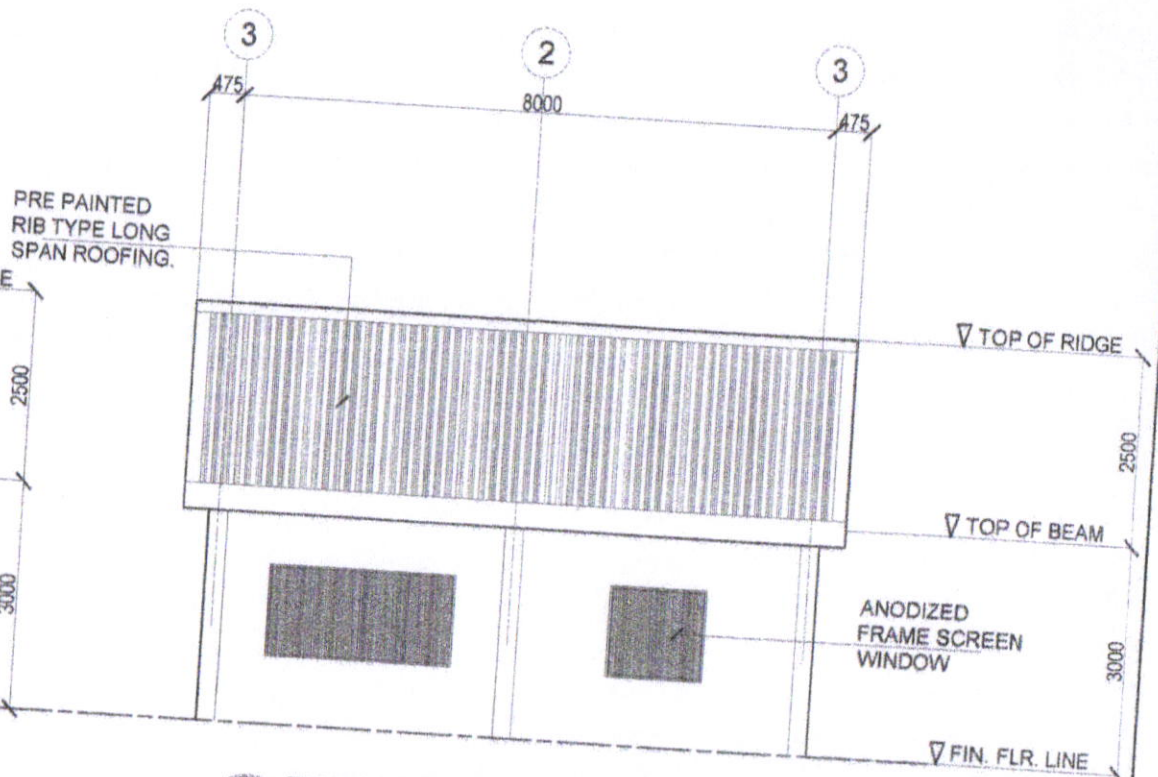
RIGHT SIDE ELEVATION SCALE : 1:100M.
