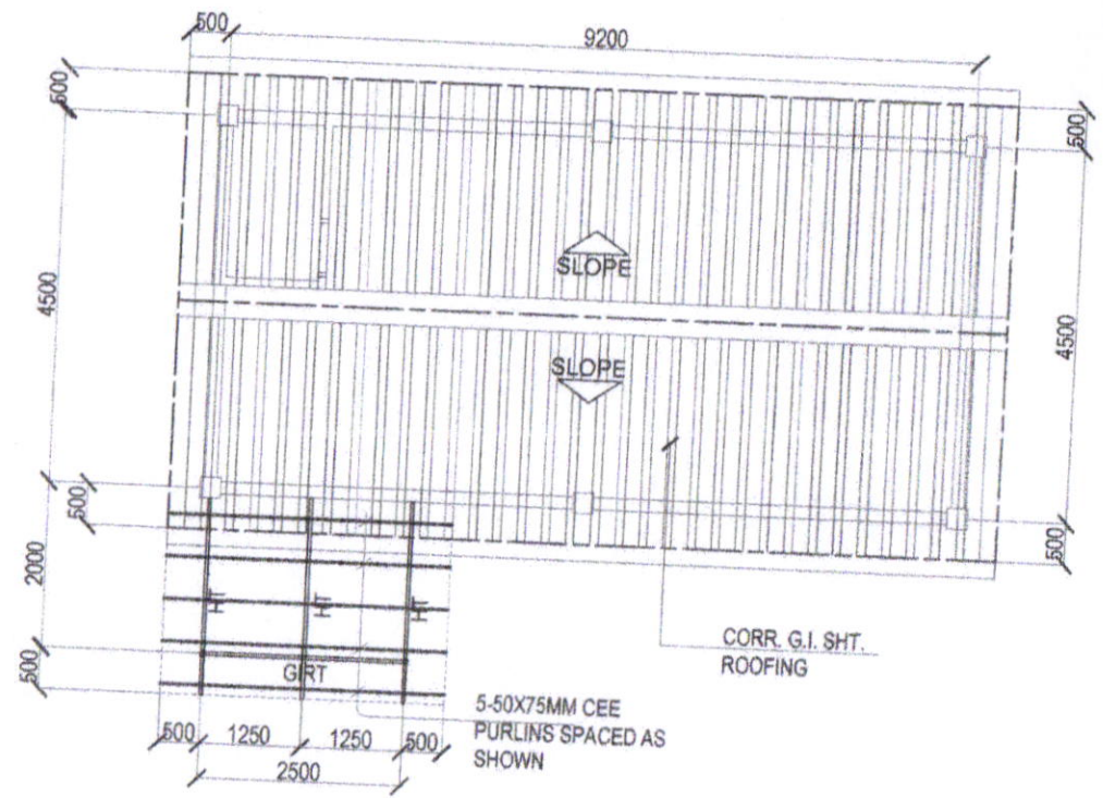
ROOF PLAN / ROOF FRAMING PLAN SCALE : 1:100M.
