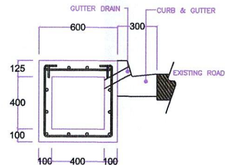
TYPICAL CANAL 3 SEC. w/ FIXED COVER
