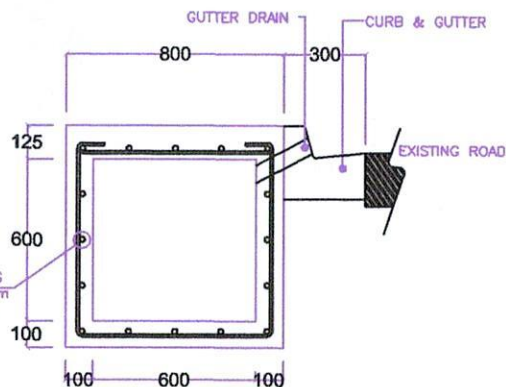
TYPICAL CANAL 2 SEC. w/ FIXED COVER
