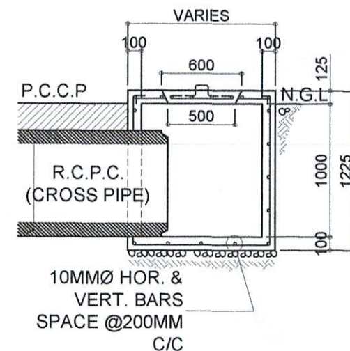
CATCH BASIN W/ R.C.P.C. SECTION ELEVATION
