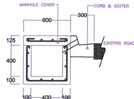
TYPICAL CANAL 3 SEC. w/ MANHOLE COVER
