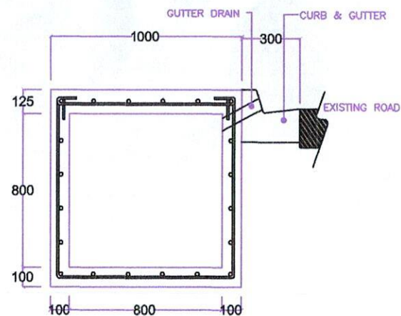
TYPICAL CANAL 1 SEC. w/ FIXED COVER
