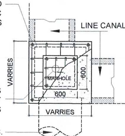
CATCH BASIN PLAN W/ R.C.P.C.
