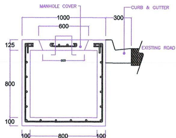
TYPICAL CANAL 1 SEC. w/ MANHOLE COVER
