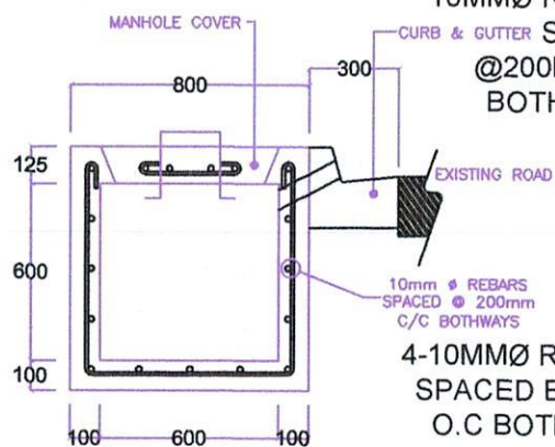
TYPICAL CANAL 2 SEC. w/ MANHOLE COVER
