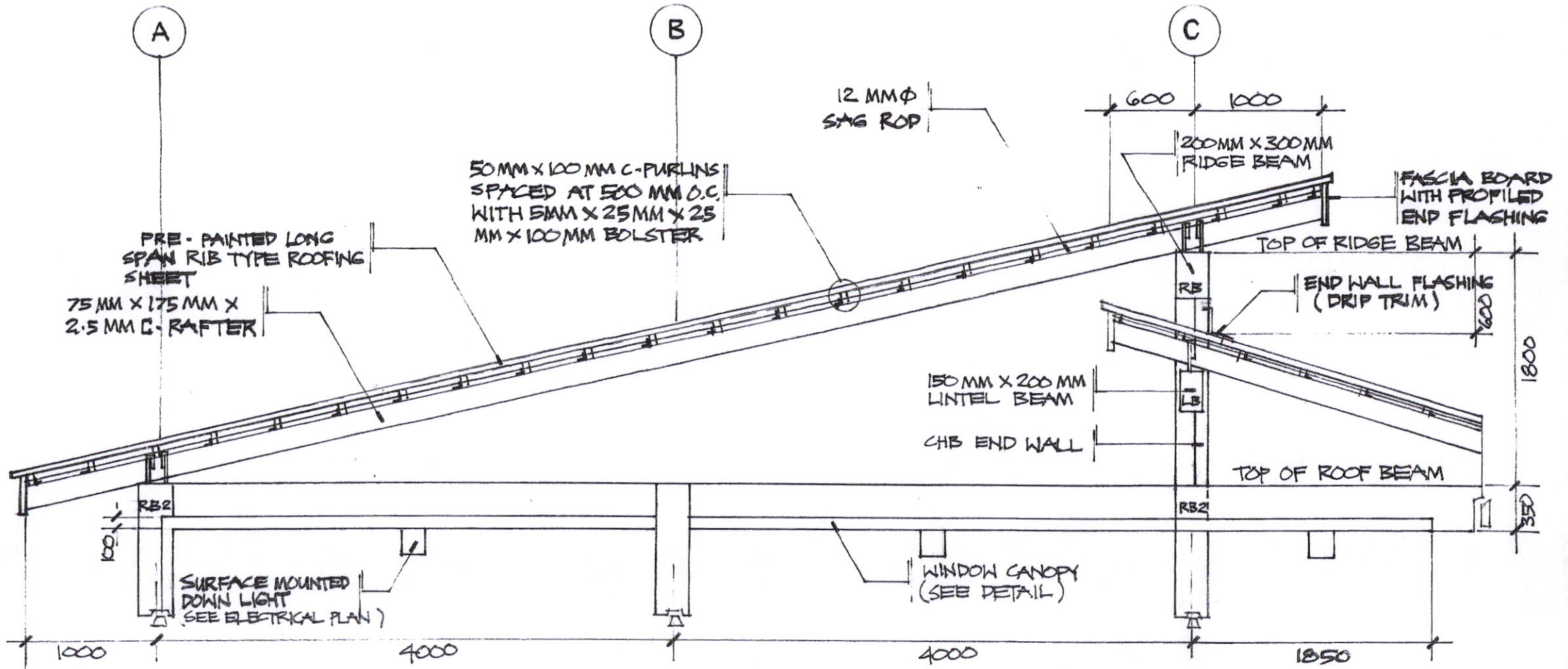
TYPICAL RAFTER DETAIL SCALE 1:40 M
