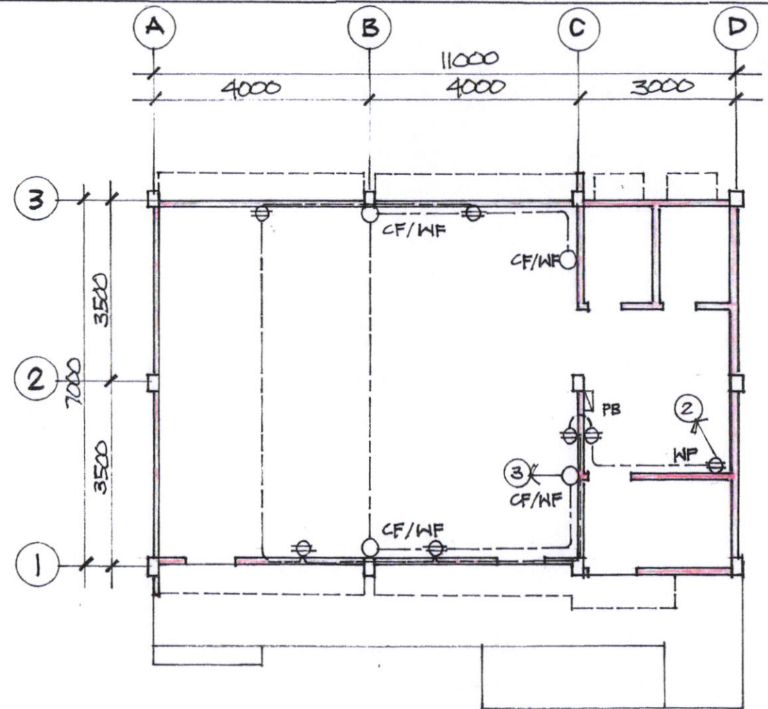
POWER LAYOUT SCALE 1:100 M
