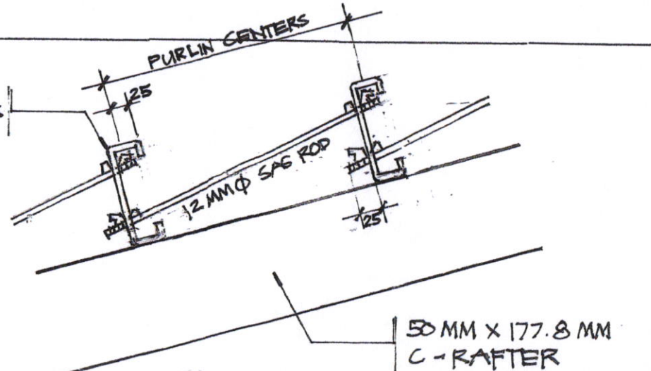
ANTI-SAG ROD DETAIL NOT TO SCALE
