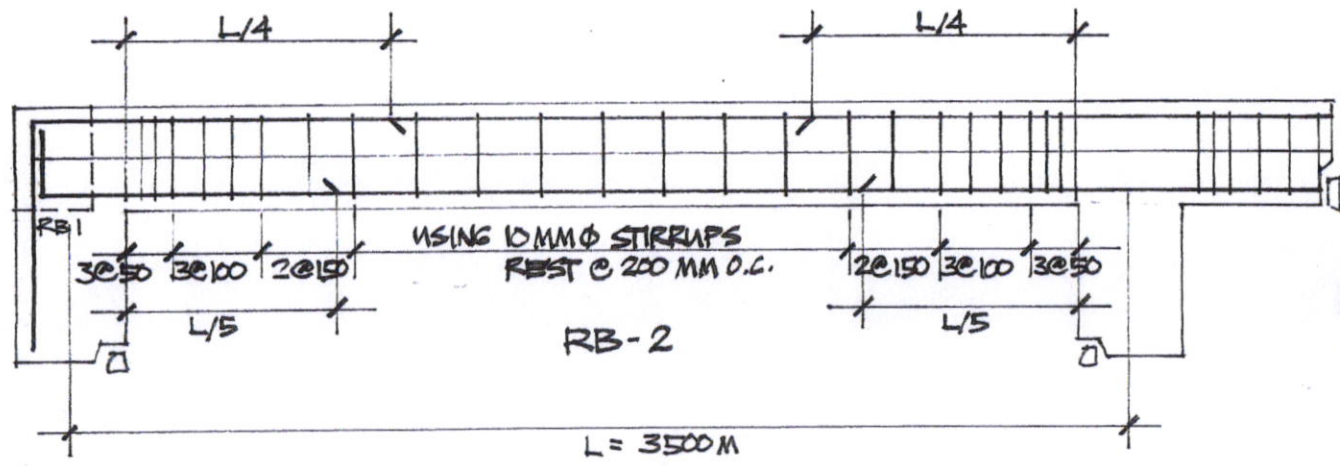
ROOF BEAM DETAIL SCALE 1:25 M
