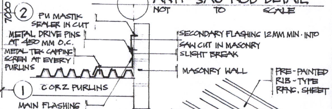
ROOF FLASHING DETAIL NOT TO SCALE
