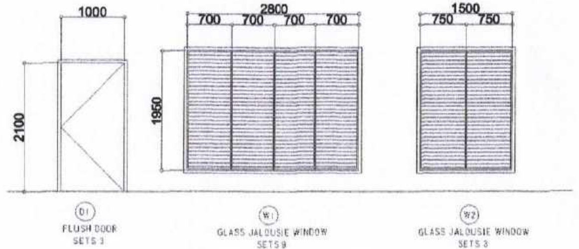
DOORS & WINDOWS SCHEDULE SCALE: 1/4"=1'-0"
