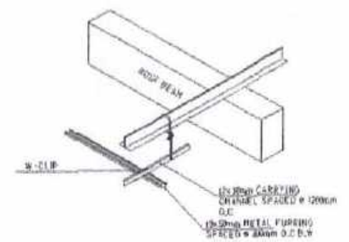
ISOMETRIC DRAWING
