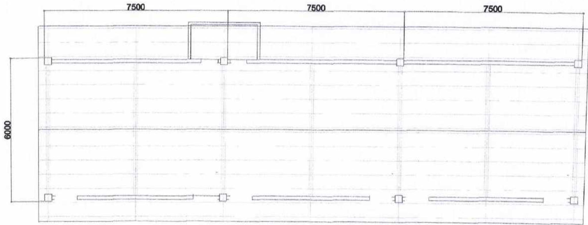
ROOF FRAMING PLAN SCALE: 1/200
