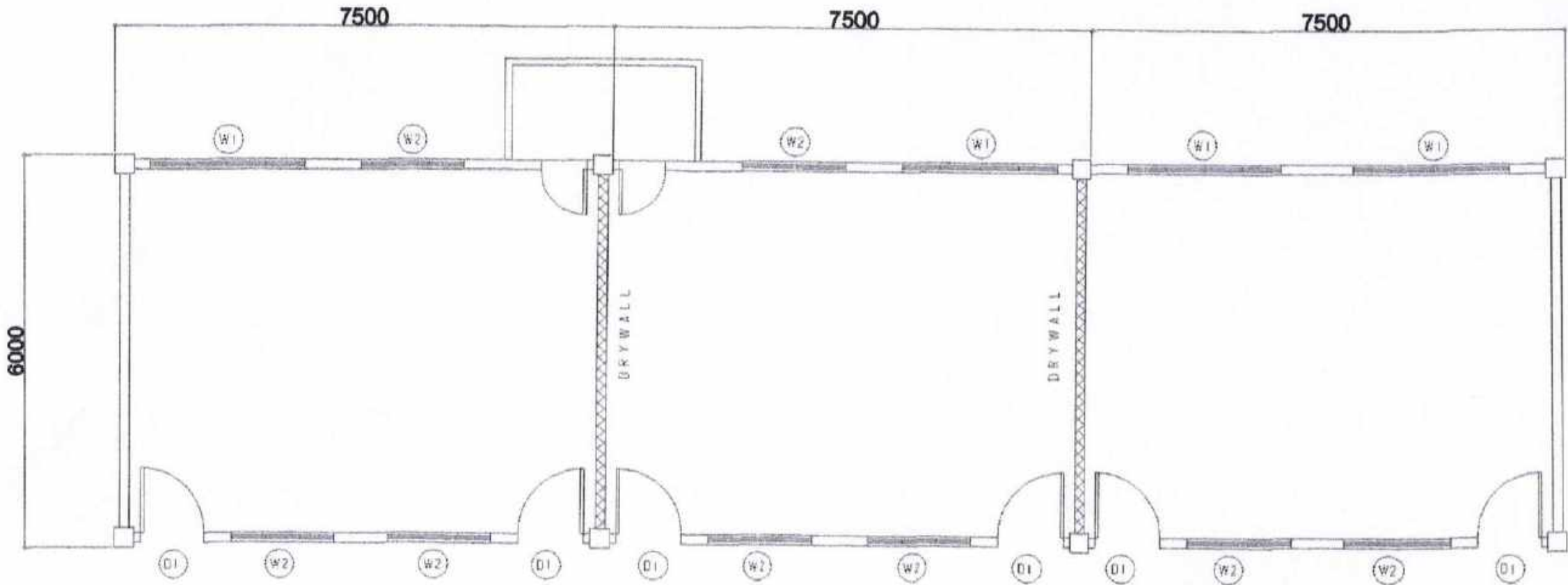
EXISTING FLOOR PLAN SCALE: 1/8" = 1'-0"
