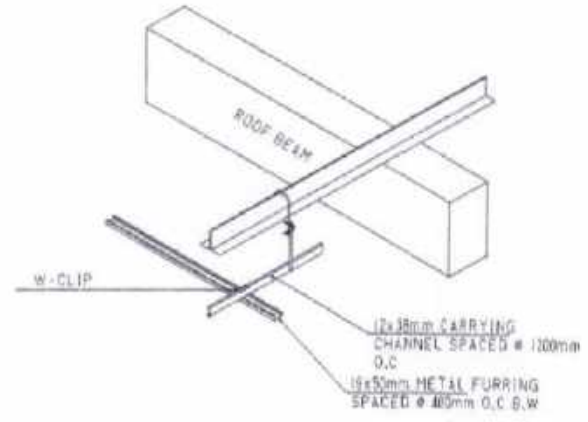
ISOMETRIC DRAWING
