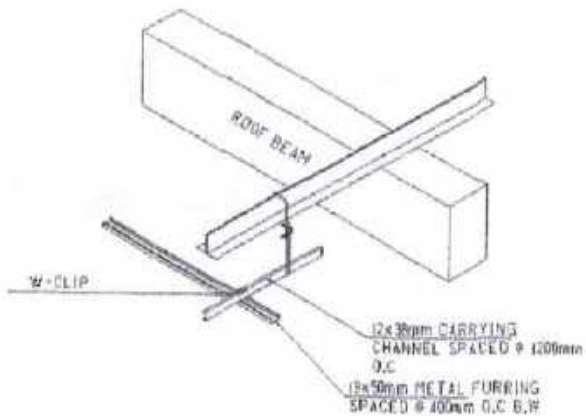
ISOMETRIC DRAWING
