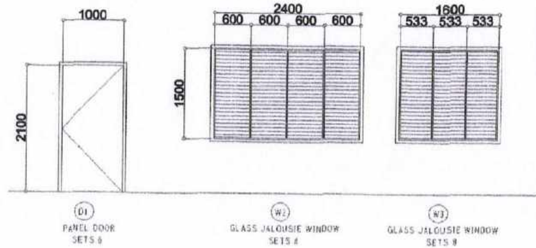
DOORS & WINDOWS SCHEDULE SCALE: 1:25MTS
