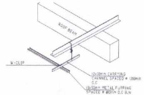
ISOMETRIC DRAWING
