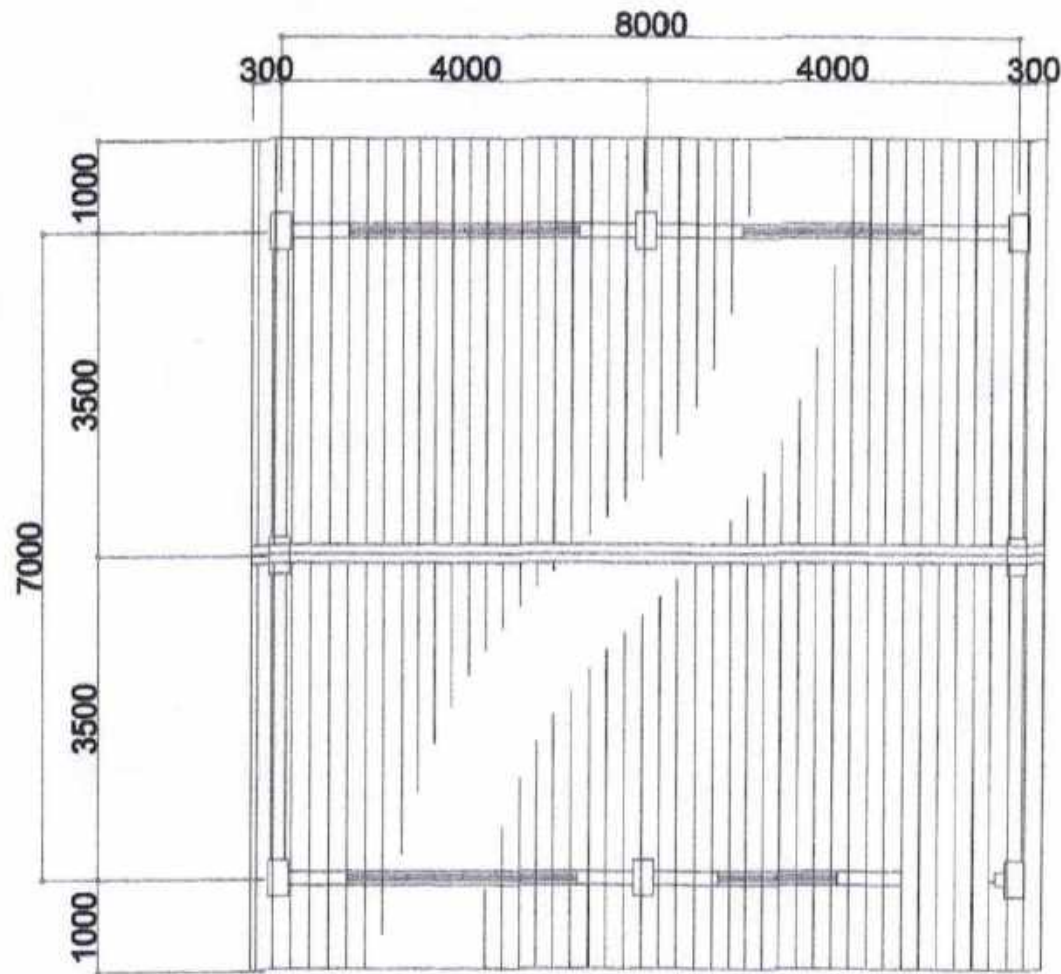
ROOF PLAN SCALE: 1/20PTS
