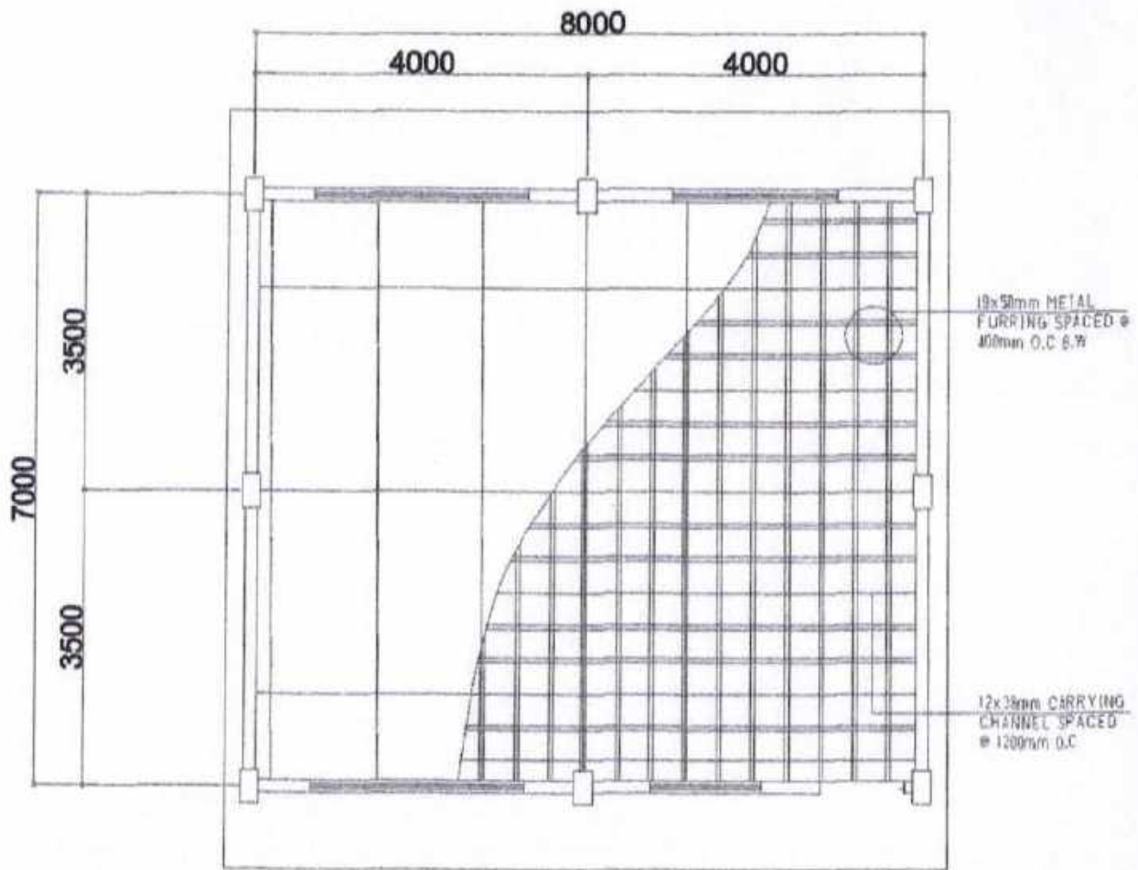
CEILING PLAN SCALE: 1/20PTS
