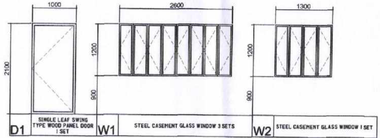
DOOR & WINDOW SCHEDULE SCALE: N T S
