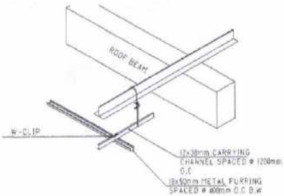
ISOMETRIC DRAWING
