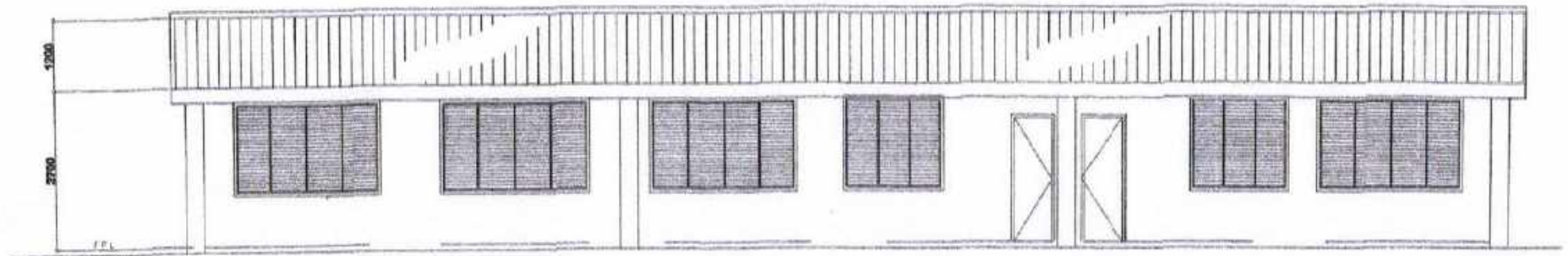
REAR ELEVATION
