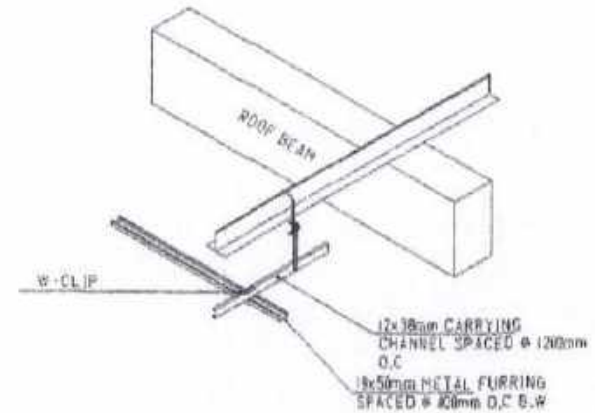
ISOMETRIC DRAWING
