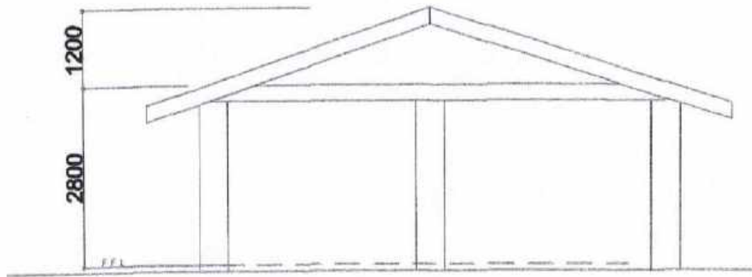
RIGHT SIDE ELEV. SCALE: 1/20PTS
