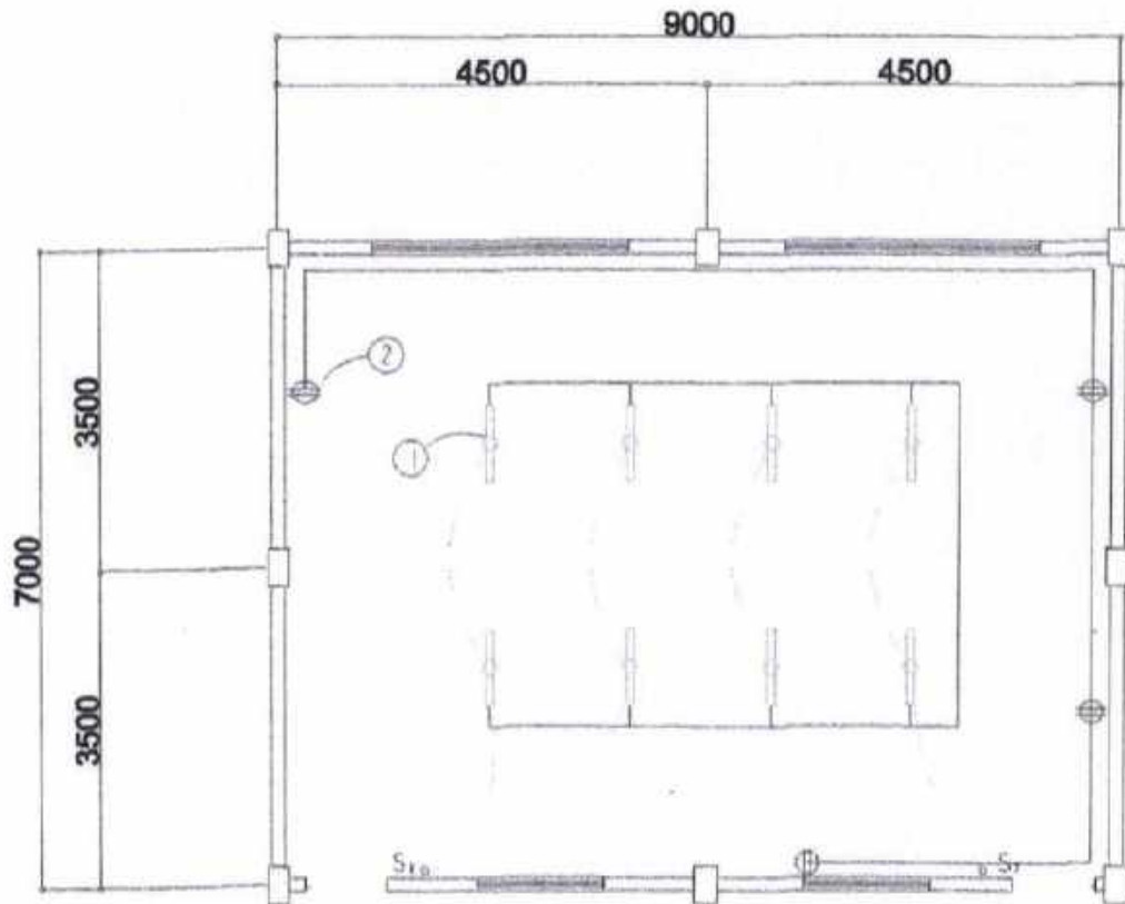
ELECTRICAL PLAN SCALE 1/8\"/>
