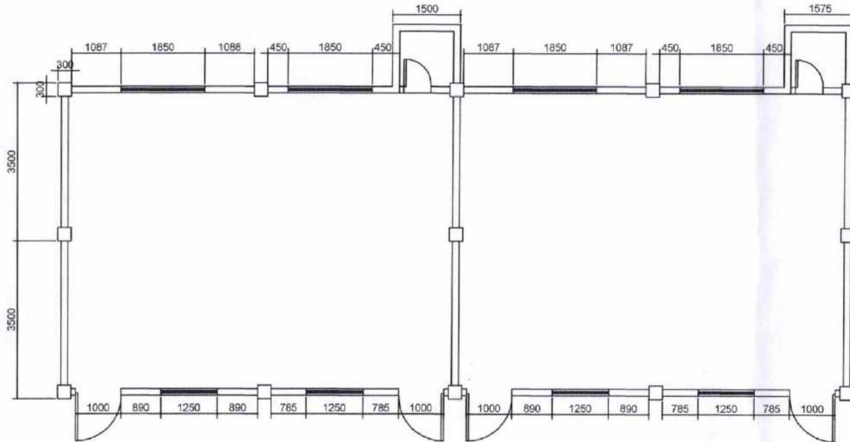
FLOOR PLAN (EXISTING) SCALE: N T S
