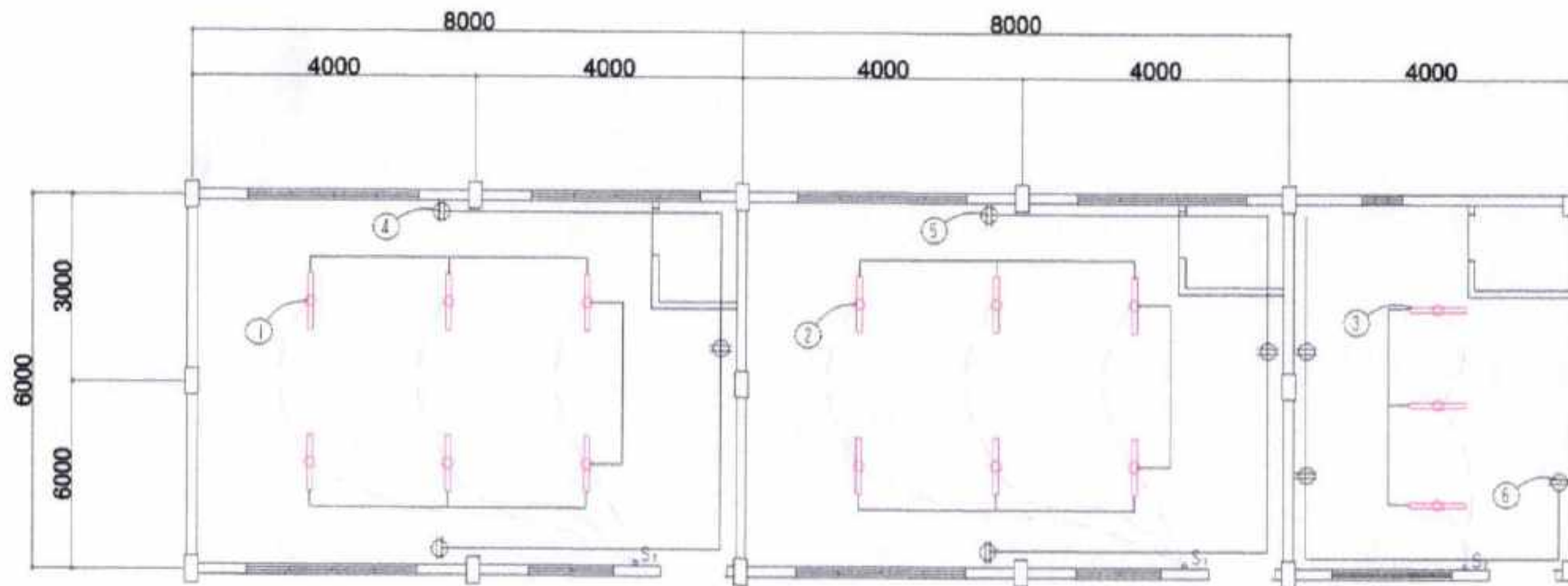
ELECTRICAL PLAN
