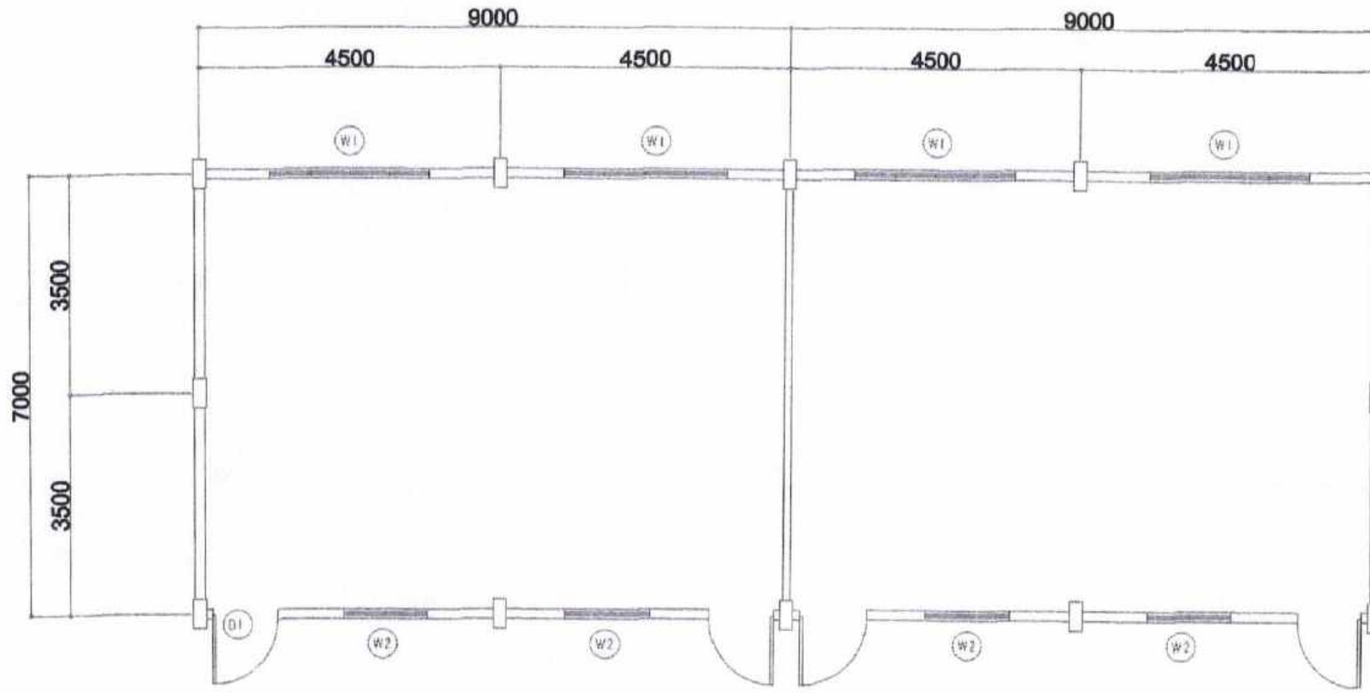
EXISTING FLOOR PLAN SCALE: 1/8" = 1'-0"
