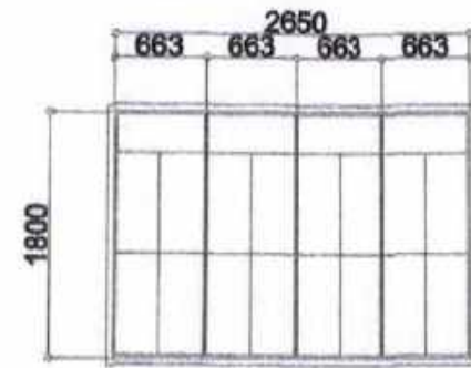
W1 STEEL CASEMENT WINDOW SETS 6
