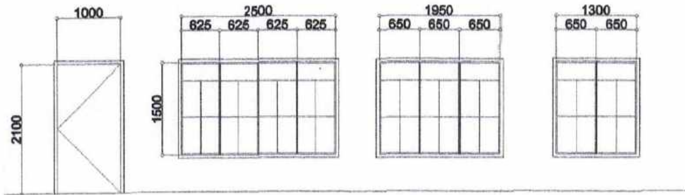
(D1) FLUSH DOOR SET 1 (W1) STEEL CASEMENT WINDOW SETS 2 (W2) STEEL CASEMENT WINDOW SET 1 (W3) STEEL CASEMENT WINDOW SET 1
