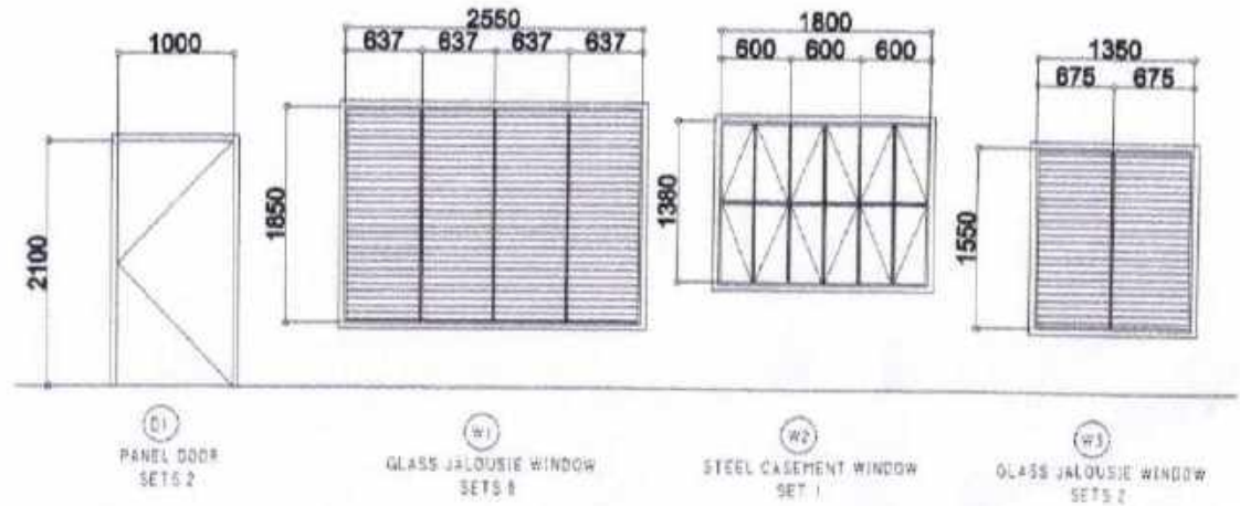
DOORS & WINDOWS SCHEDULE SCALE: 1/8"=1'-0"
