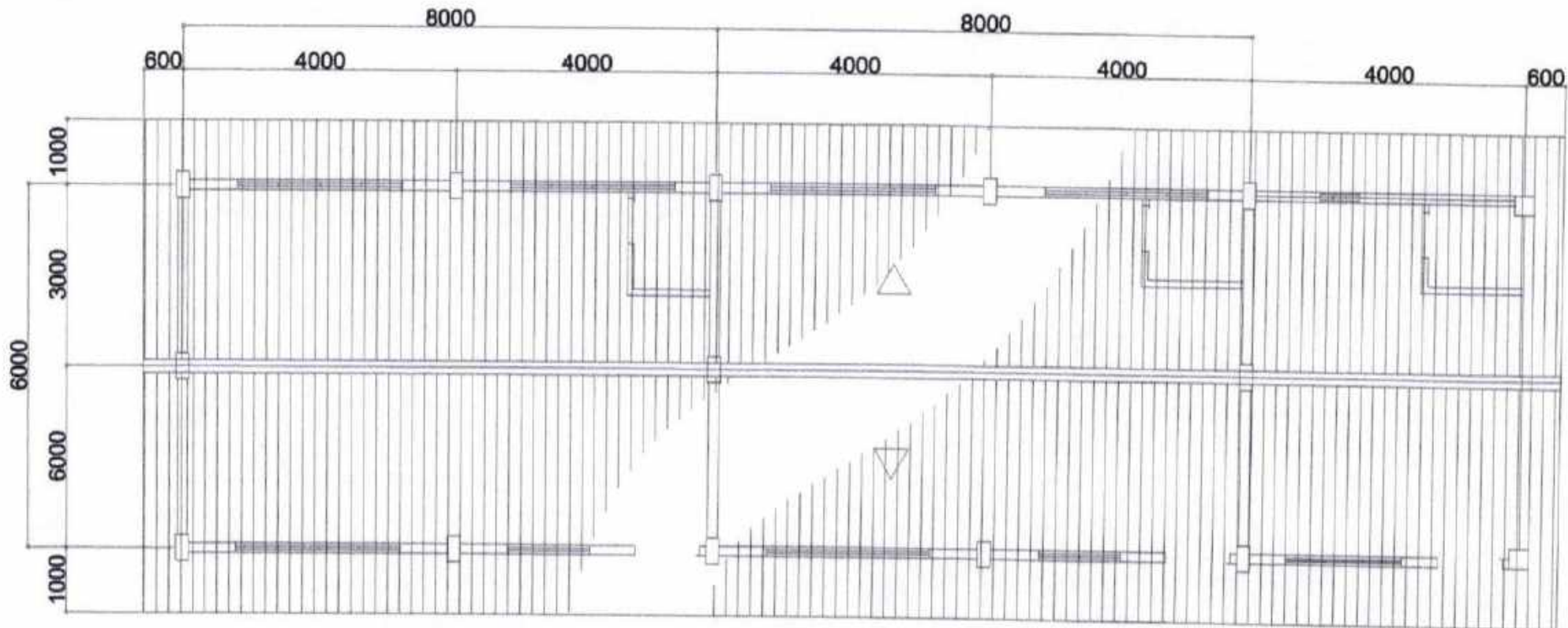
ROOF PLAN SCALE: 1/8" = 1'-0"
