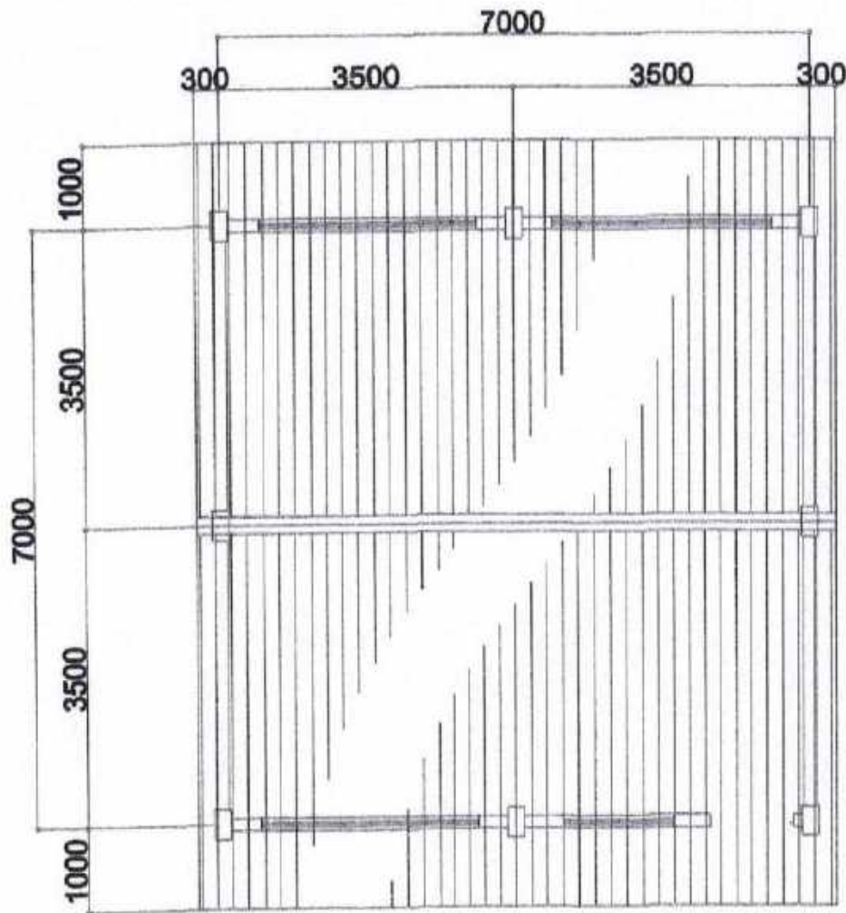
ROOF PLAN SCALE 1:200
