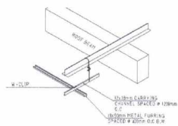
ISOMETRIC DRAWING
