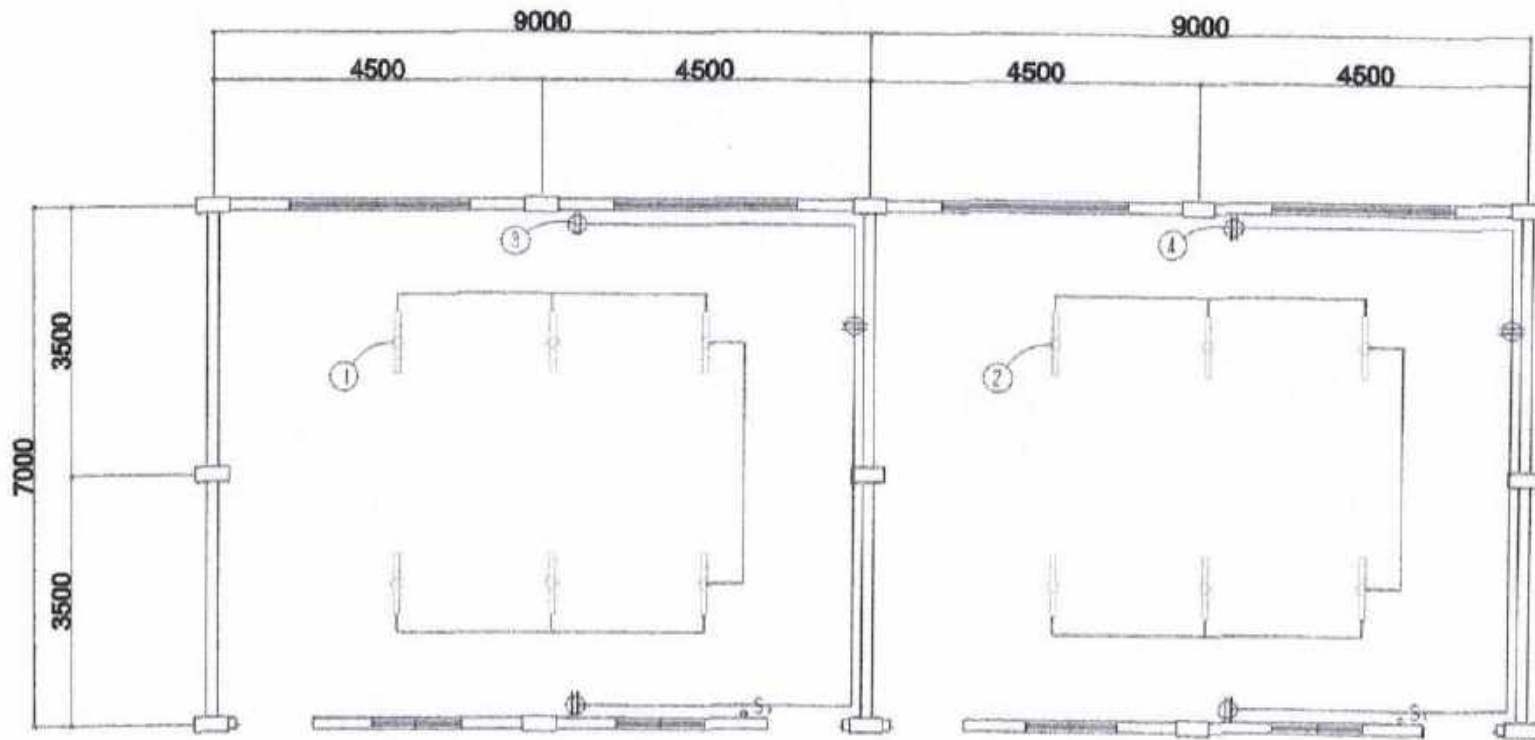
ELECTRICAL PLAN
