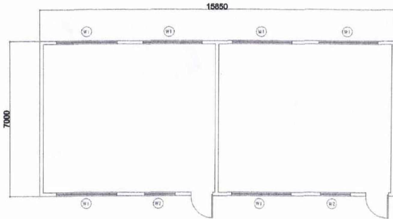
EXISTING FLOOR PLAN SCALE: 1/8"=1'-0"
