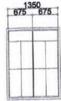
W2 STEEL CASEMENT WINDOW SETS 2
