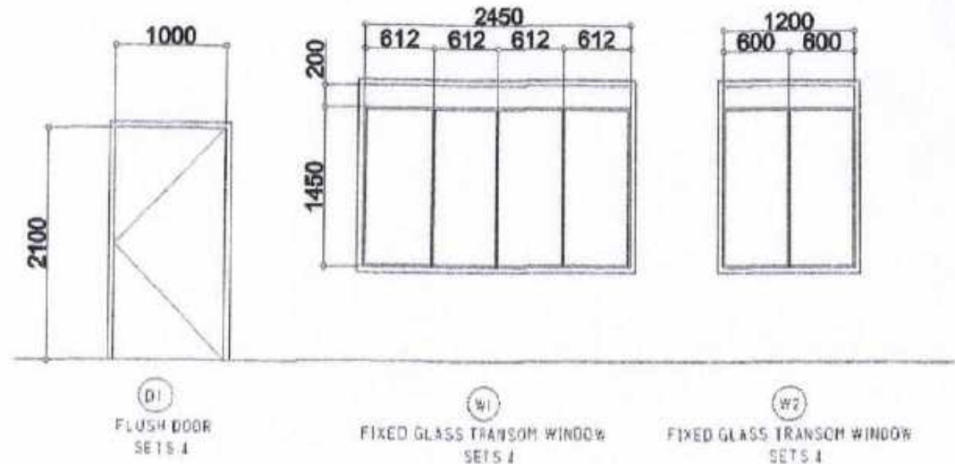
DOORS & WINDOWS SCHEDULE SCALE: 1:25RTS
