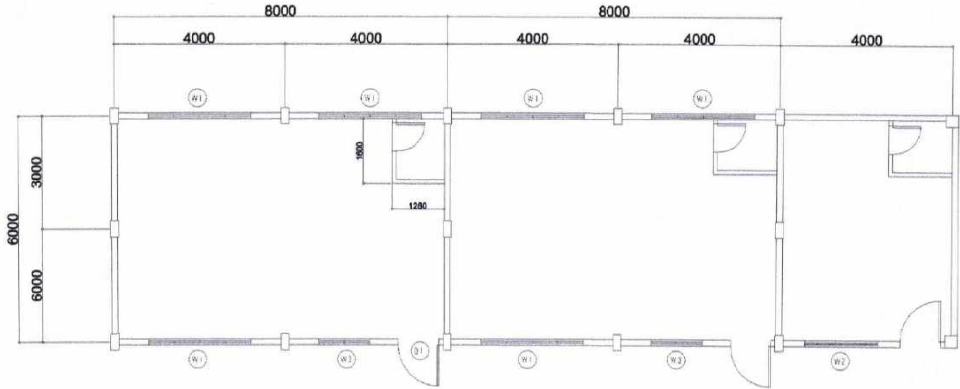
EXISTING FLOOR PLAN SCALE: 1/8"=1'-0"
