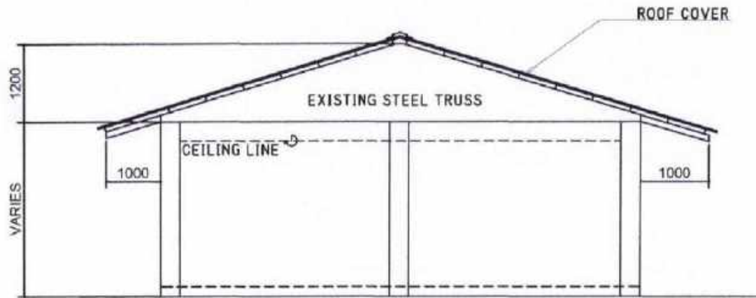
○ SIDE ELEVATION SCALE: N T S
