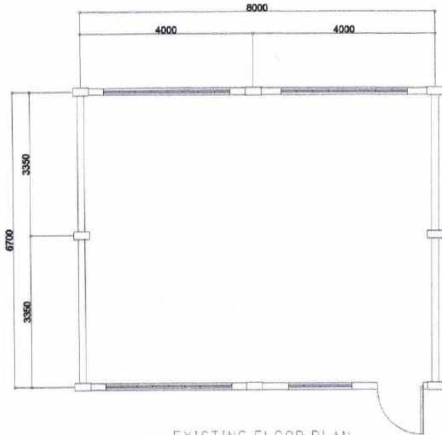
EXISTING FLOOR PLAN SCALE: 1/8"=1'-0"
