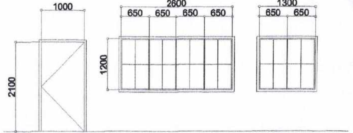
(D1) FLUSH DOOR SET 1 (W1) STEEL CASEMENT WINDOW SETS 3 (W2) STEEL CASEMENT WINDOW SET 1
