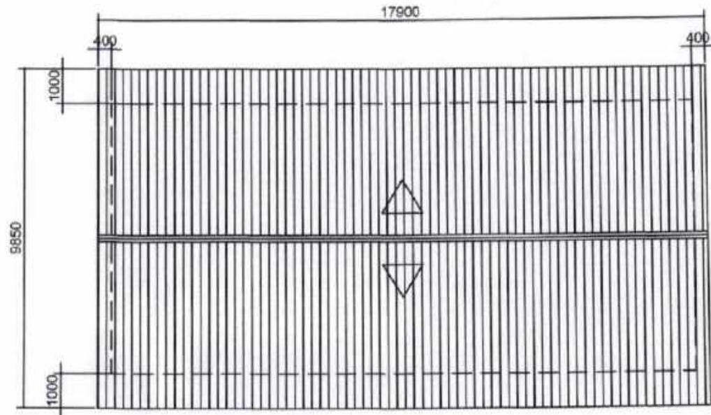
ROOF PLAN SCALE: N T S
