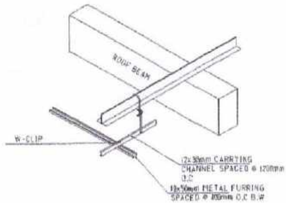
ISOMETRIC DRAWING
