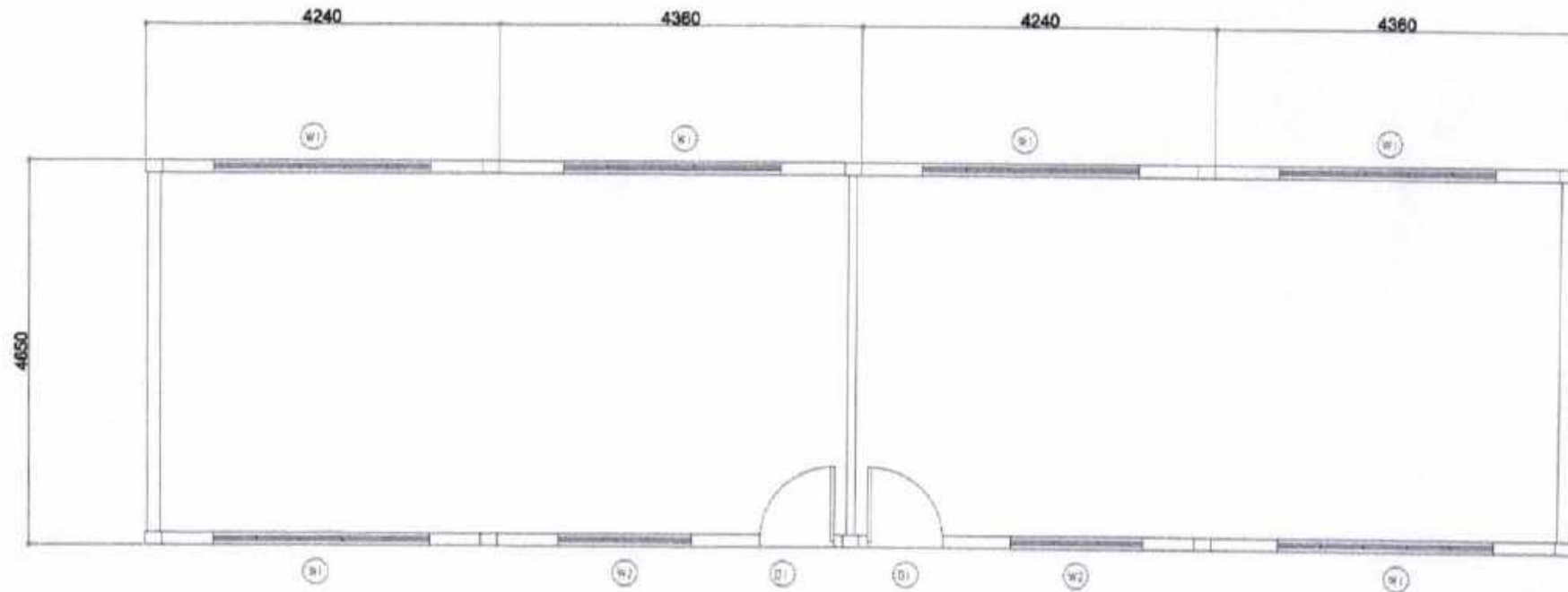
EXISTING FLOOR PLAN SCALE 1:200
