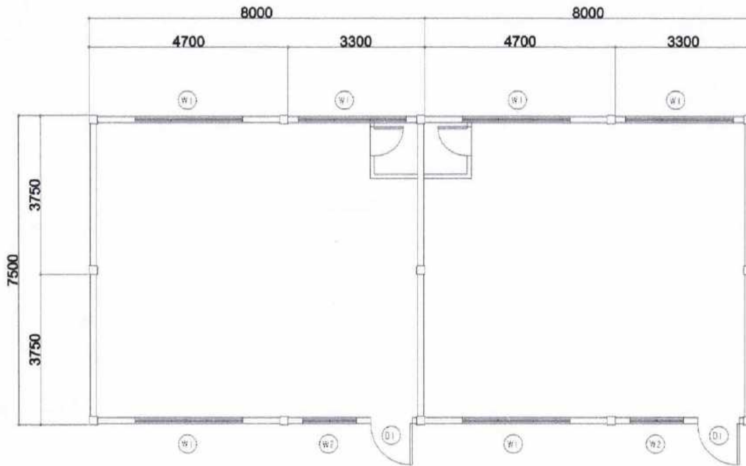
EXISTING FLOOR PLAN SCALE: 1:50
