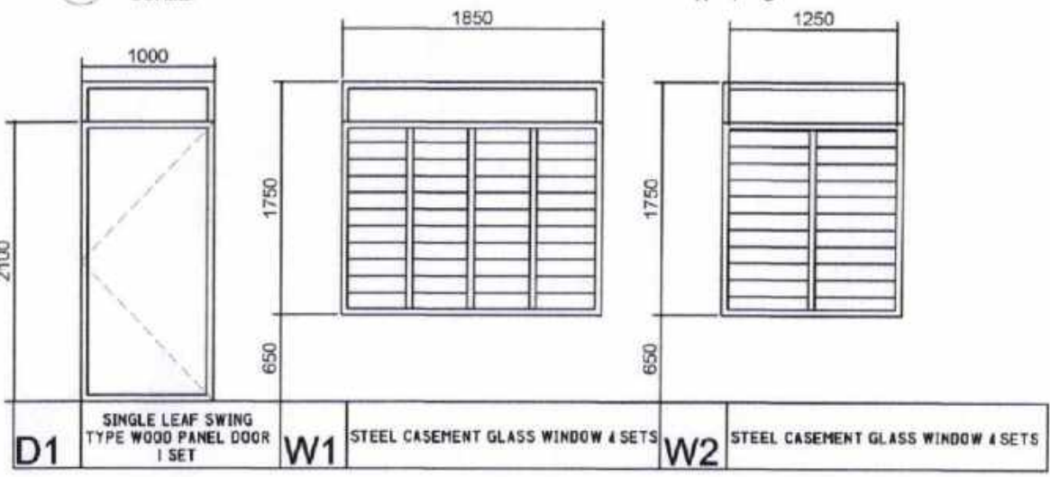
DOOR & WINDOW SCHEDULE SCALE: N T S
