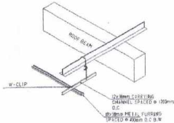
ISOMETRIC DRAWING
