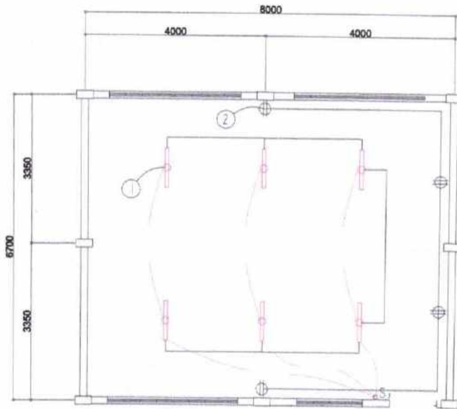
ELECTRICAL PLAN
