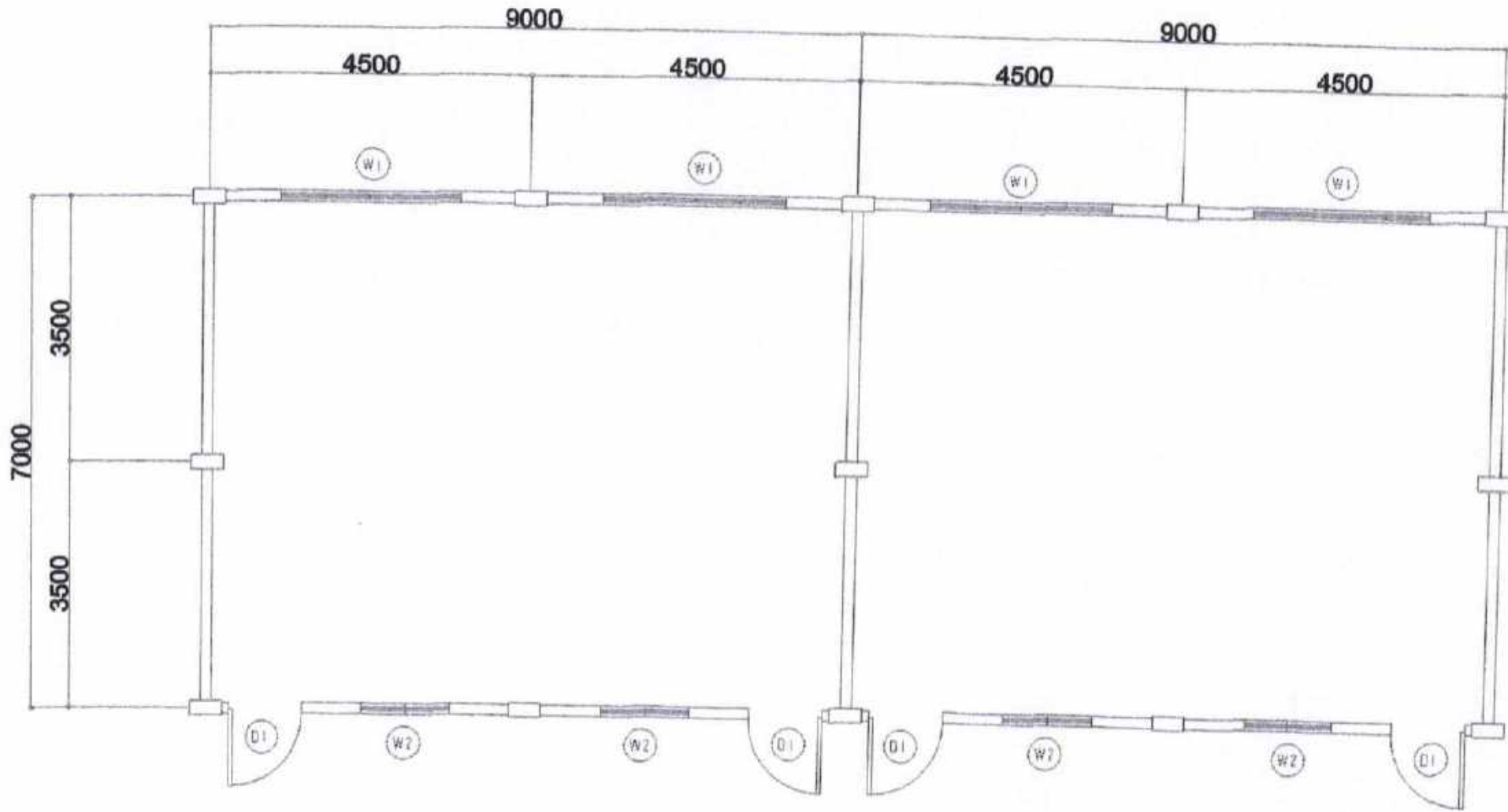
EXISTING FLOOR PLAN SCALE 1:300
