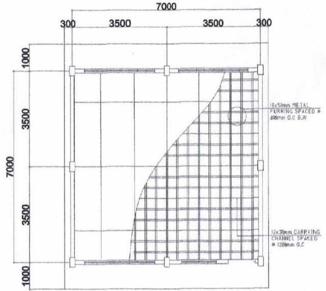
CEILING PLAN SCALE 1:200
